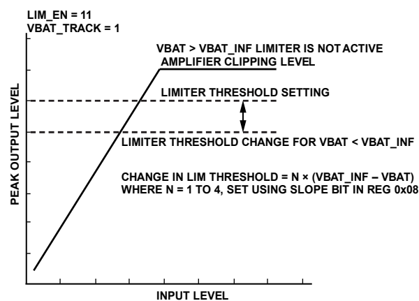
Figure 73. Limiter Example (LIM_EN = 0b11, VBAT_TRACK = 0b1)
