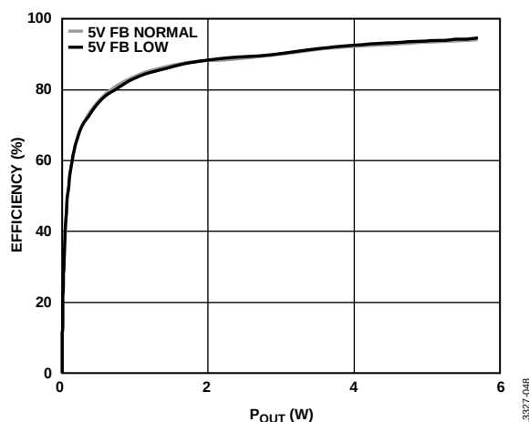
Figure 54. Efficiency vs. P_{OUT} , R_L = 3\ \Omega , FB and 220 pF Capacitor, PV_{DD} = 5\text{ V} , Analog Gain = 8.4
