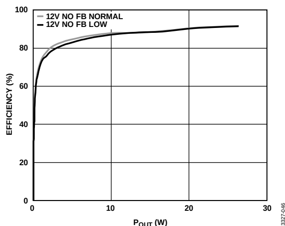
Figure 52. Efficiency vs. P_{OUT} , R_L = 3\ \Omega , No FB and 220 pF Capacitor, PV_{DD} = 12\text{ V} , Analog Gain = 12.6
