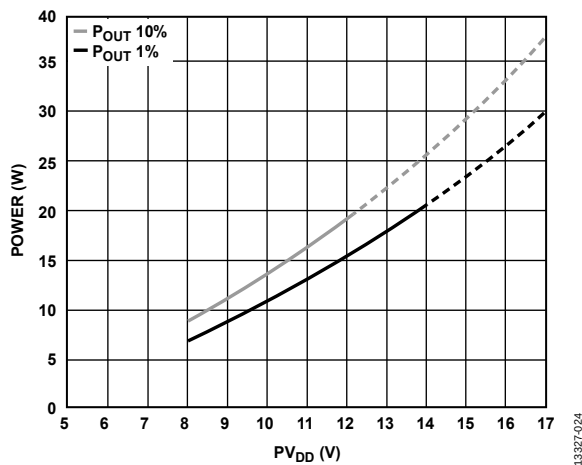
Figure 32. Output Power vs. P_{VDD} , R_L = 4\ \Omega , Analog Gain = 15
