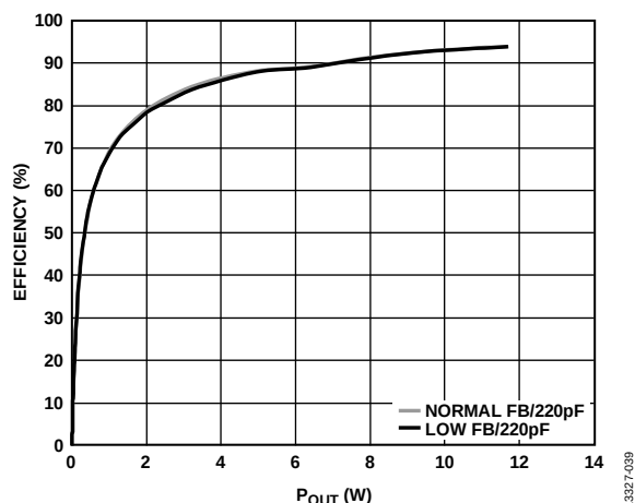
Figure 49. Efficiency vs. P_{OUT} , R_L = 8\ \Omega , FB and 220 pF Capacitor, PV_{DD} = 12\text{ V} , Analog Gain = 12.6
