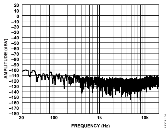
Figure 10. FFT, 60 dBFS Input, Analog Gain = 15, R_L = 4\ \Omega
