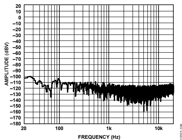
Figure 12. FFT, No Signal, Analog Gain = 12.6, R_L = 4\ \Omega
