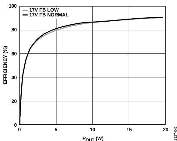
Figure 50. Efficiency vs. P_{OUT} , R_L = 8\ \Omega , FB and 220 pF Capacitor, PV_{DD} = 17\text{ V} , Analog Gain = 14
