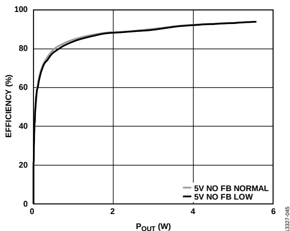
Figure 51. Efficiency vs. P_{OUT} , R_L = 3\ \Omega , No FB and 220 pF Capacitor, PV_{DD} = 5\text{ V} , Analog Gain = 8.4
