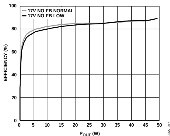
Figure 53. Efficiency vs. P_{OUT} , R_L = 3\ \Omega , No FB and 220 pF Capacitor, PV_{DD} = 17\text{ V} , Analog Gain = 14
