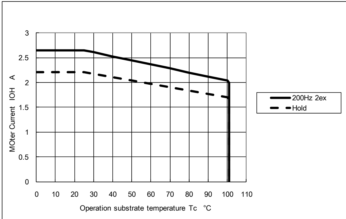
Derating Curve of Motor Current, I_{OH} , vs. STK672-630CN-E Operating Substrate Temperature, T_c
