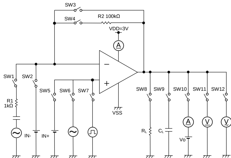
Figure 25. Test Circuit 2
