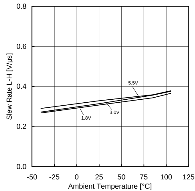
Figure 21. Slew Rate L-H vs Ambient Temperature
