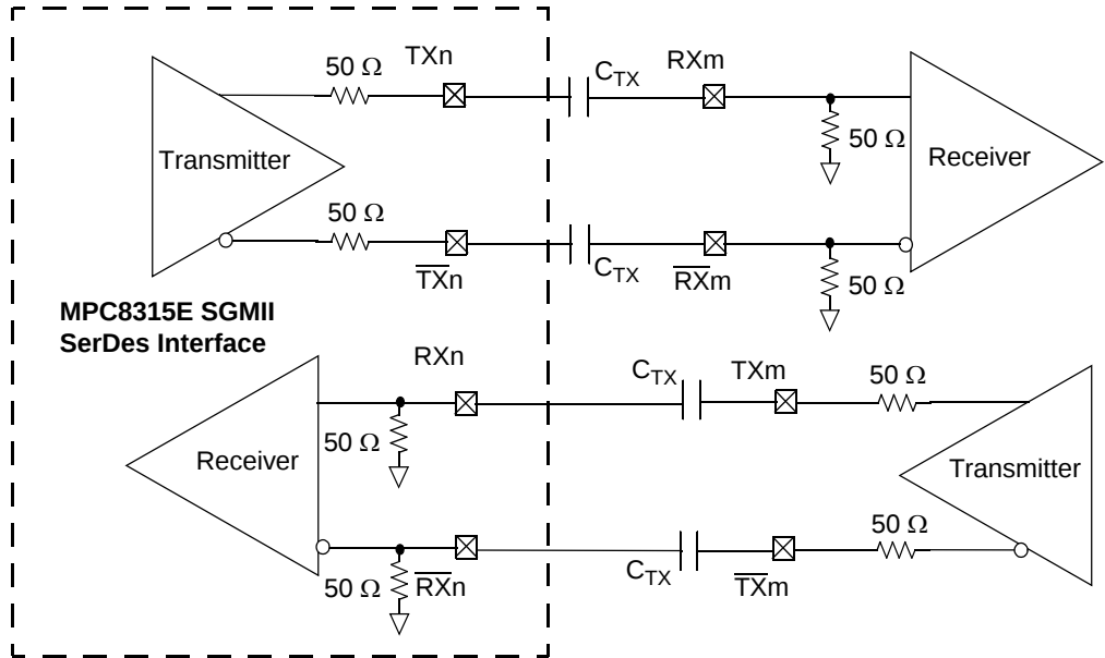
Figure 18. 4-Wire AC-Coupled SGMII Serial Link Connection Example
