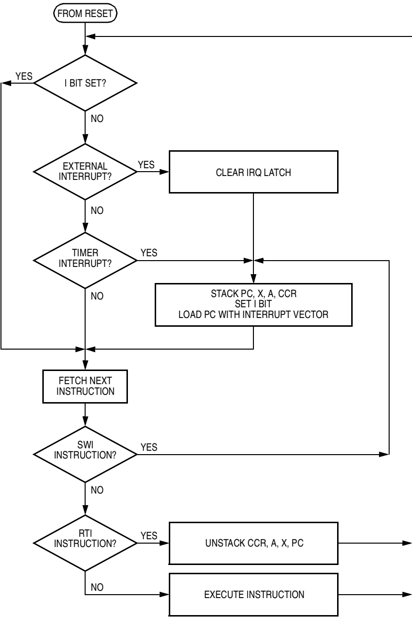
Figure 4-7. Interrupt Flowchart
