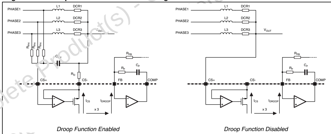
Figure 8. Droop Function Current Reading Network
