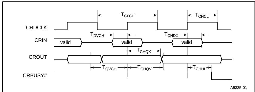
Figure 11. Serial Debug Unit
