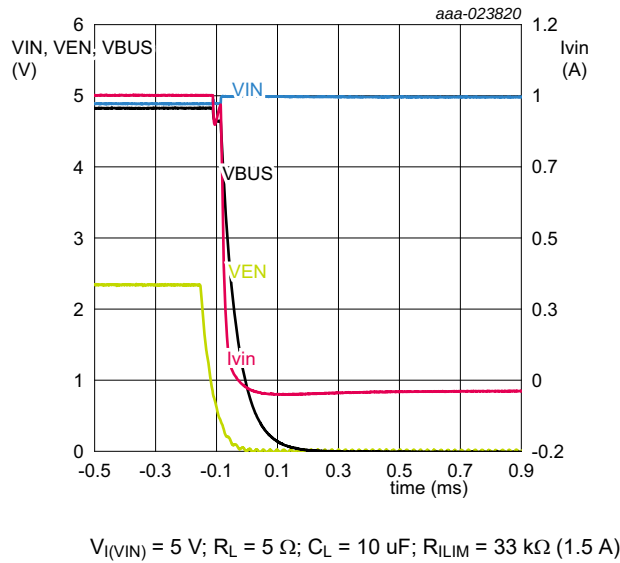
Fig 16. Typical 10 uF disable time
