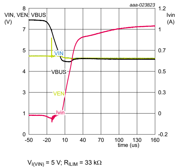
Fig 19. Reverse-current protection recovery
