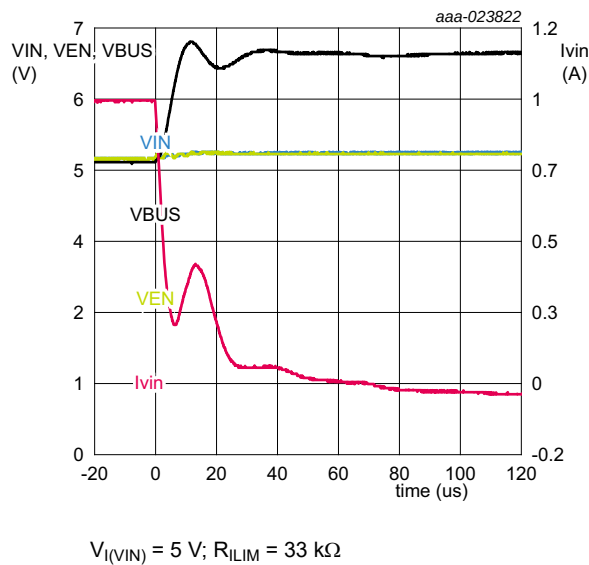
Fig 18. Reverse-current protection response
