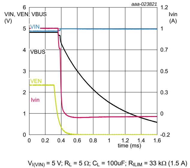
Fig 17. Typical 100 uF disable time
