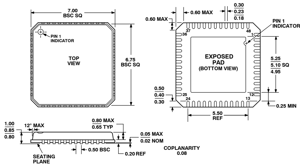
COMPLIANT TO JEDEC STANDARDS MO-220-VKGD-2 Figure 48. 48-Lead Lead Frame Chip Scale Package [LFCSP_VQ] 7 mm x 7 mm Body, Very Thin Quad (CP-48-1) Dimensions shown in millimeters
