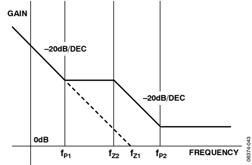
Figure 42. Poles and Zeros of Voltage Error Amplifier
