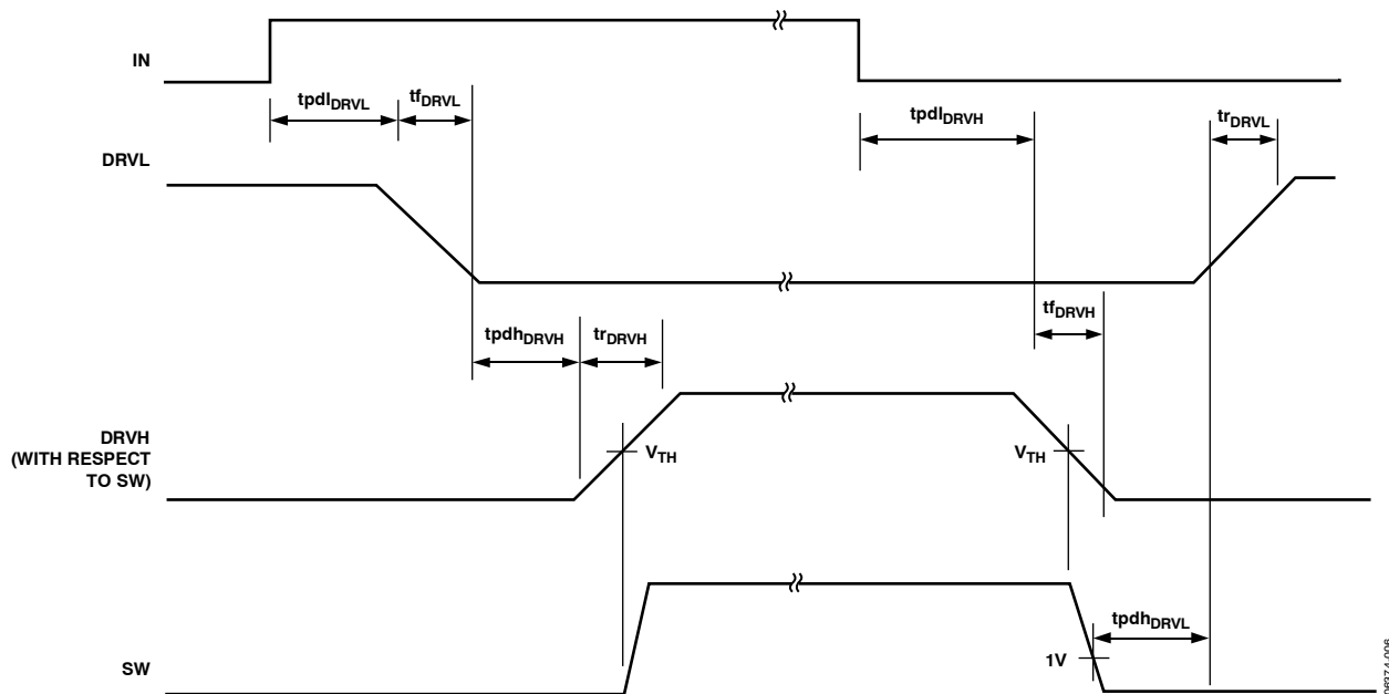
Figure 2. Timing Diagram
