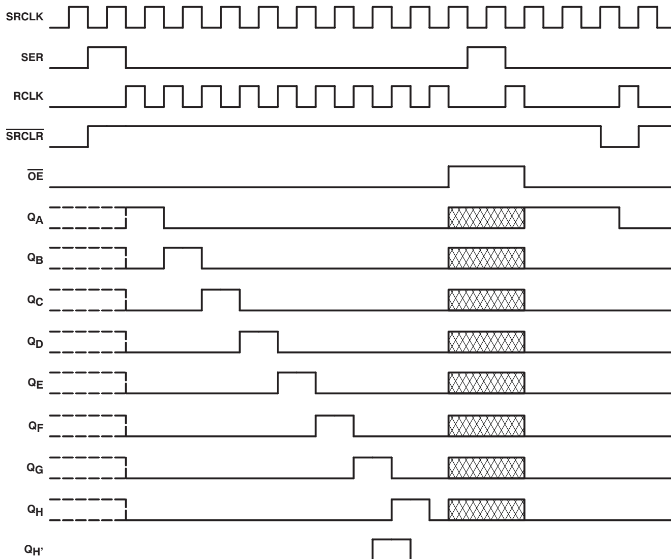
Figure 1. Timing Diagram
