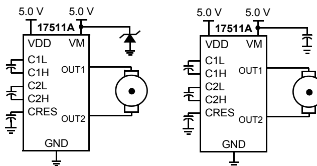
Figure 8. CEMF Snubbing Techniques
