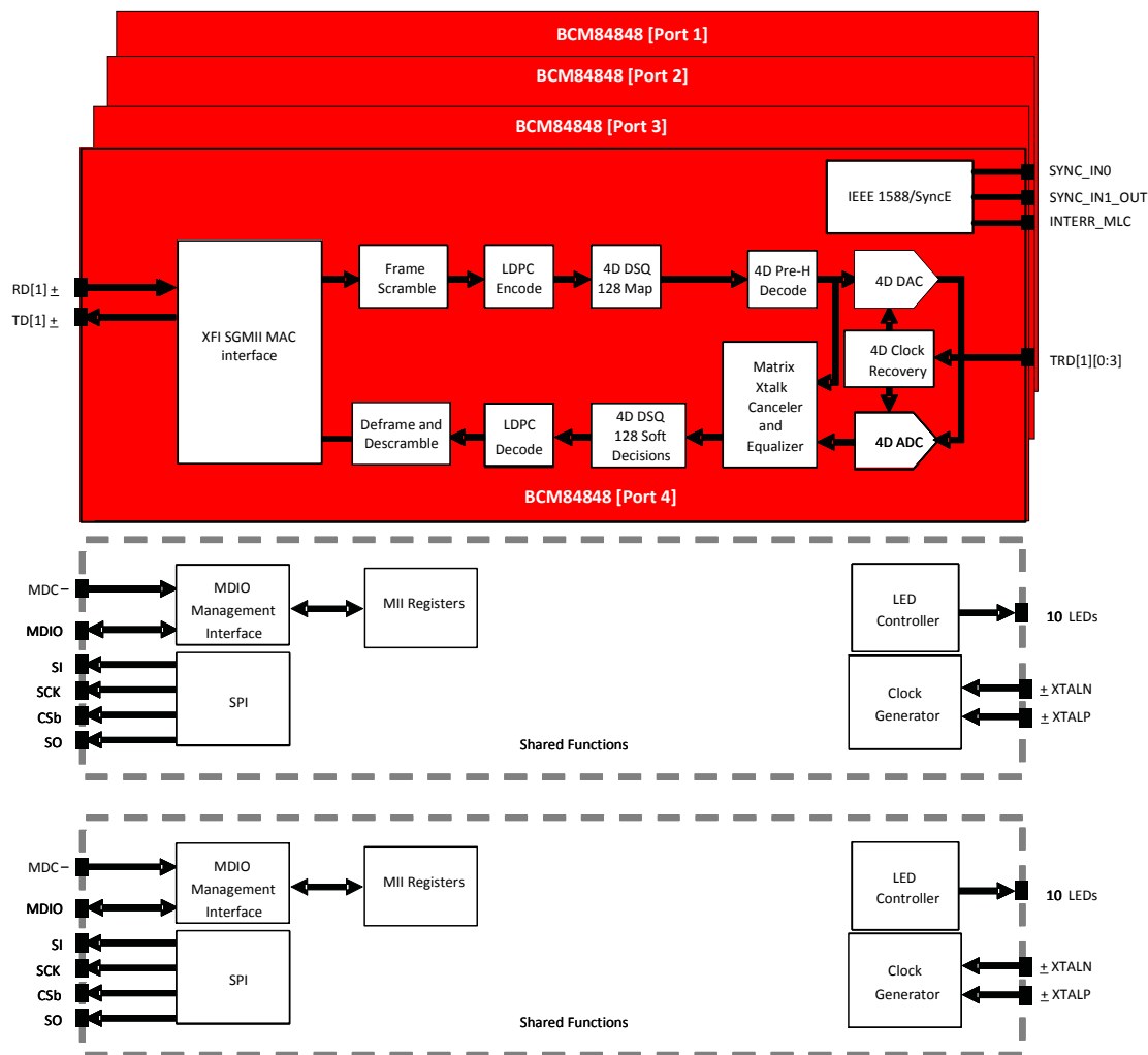
BCM84848 Block Diagram for Each Port
