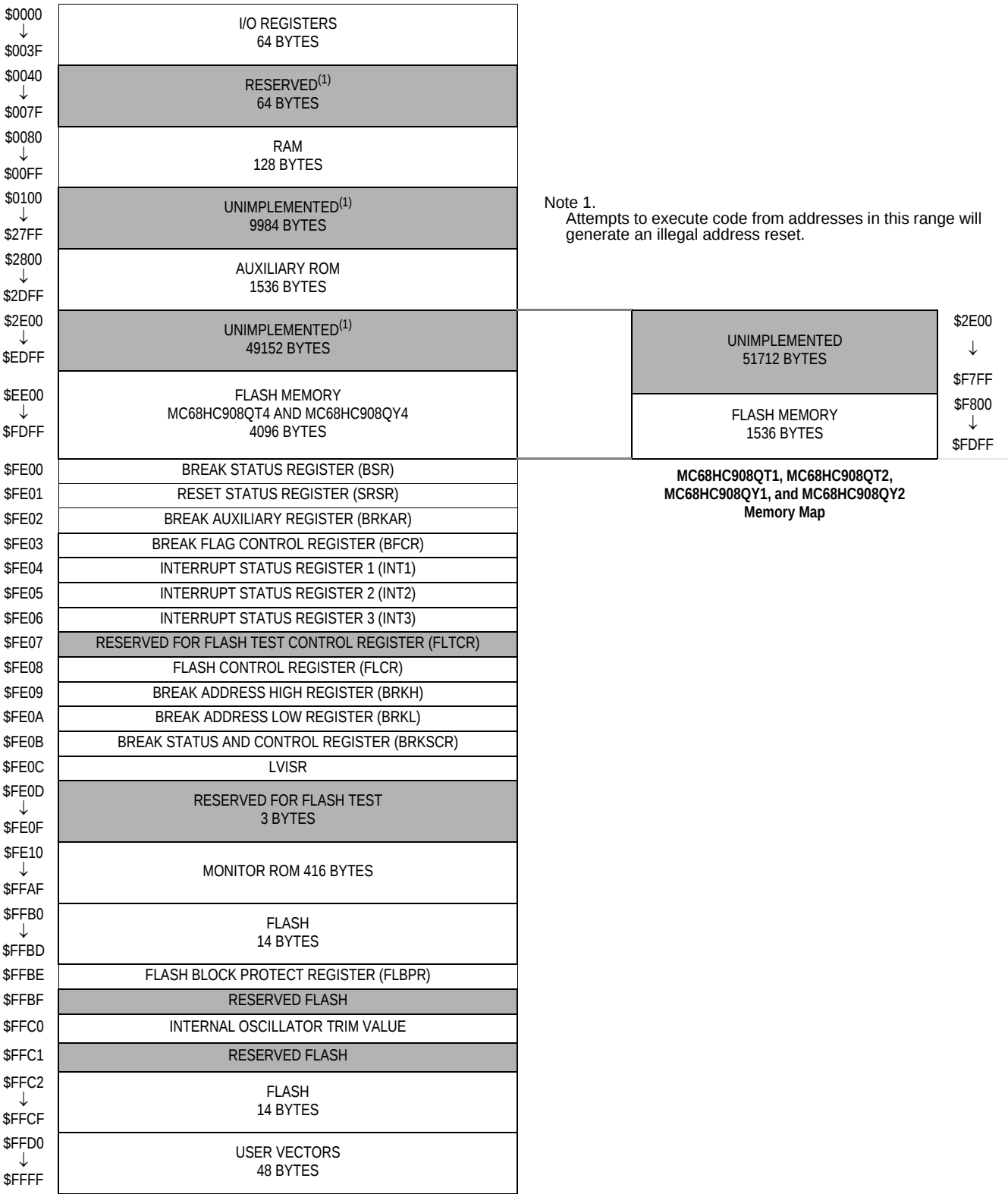
Figure 3. Memory Map
