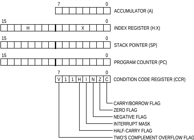
Figure 16. CPU Registers
