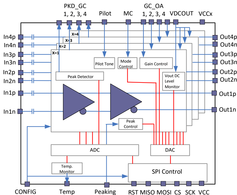
Figure 1. Block Diagram
