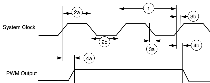
Figure 66. PWM Timing
