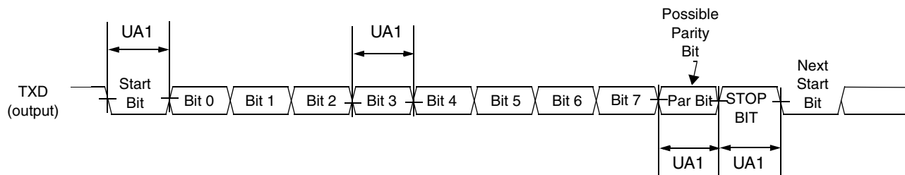
Figure 89. UART RS-232 Serial Mode Transmit Timing Diagram
