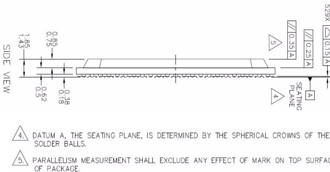
Figure 104. 19 x 19 mm Package Side View
