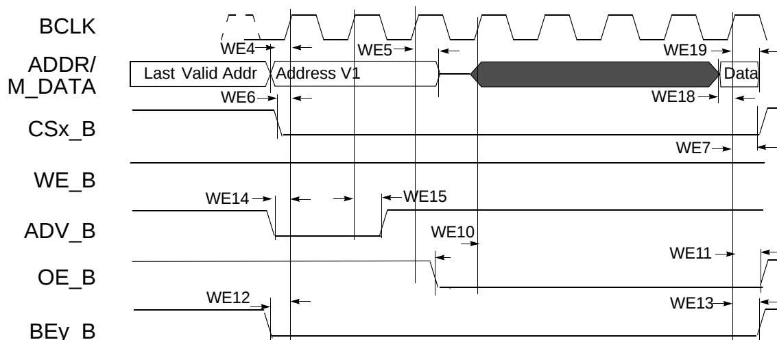
Figure 21. 16-Bit Muxed A/D Mode, Synchronous Read Access, WSC=7, RADVN=1, ADH=1, OEA=2
