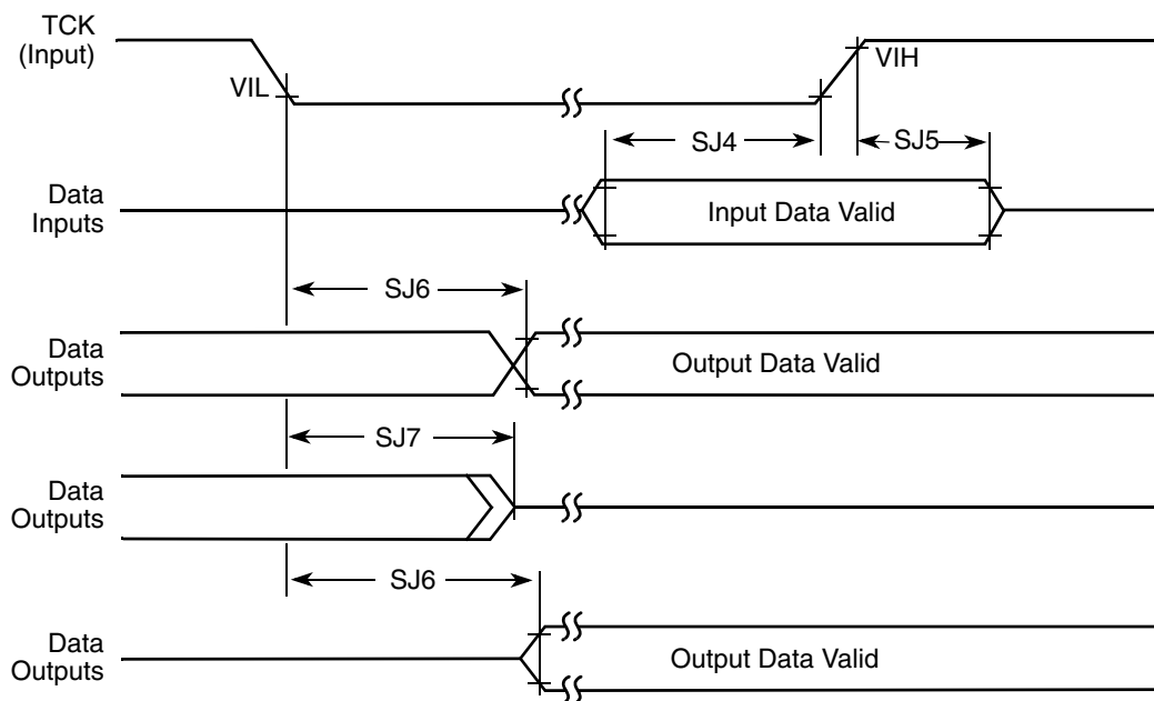
Figure 80. Boundary Scan (JTAG) Timing Diagram
