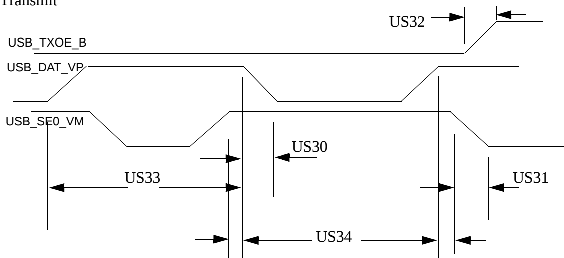
Figure 99. USB Transmit Waveform in VP_VM Unidirectional Mode
