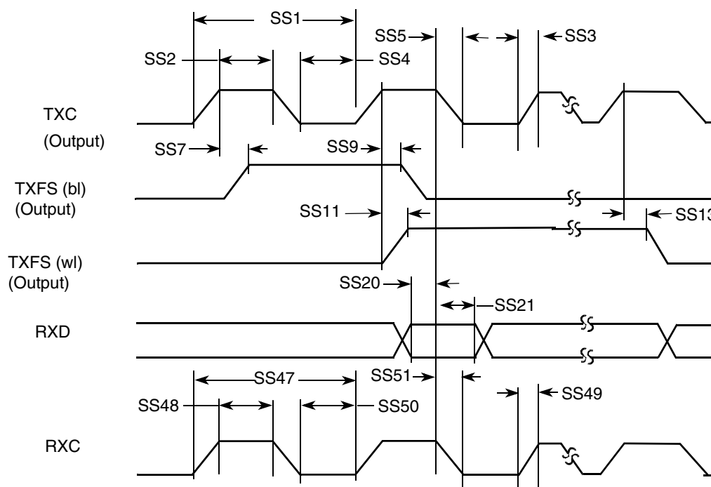
Figure 86. SSI Receiver Internal Clock Timing Diagram
