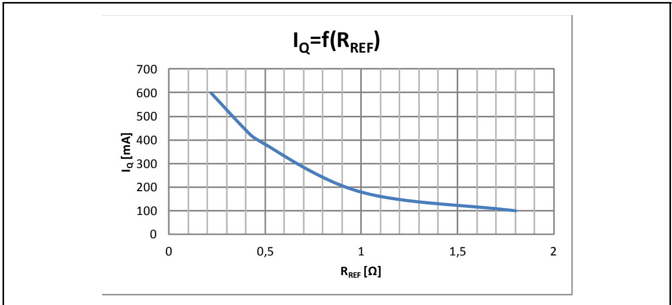
Figure 5-3 Output Current I_Q versus Reference Resistor R_{REF} with V_Q = 6.6 \text{ V}
