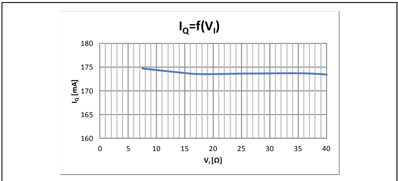
Figure 5-4 Output Current I_Q versus Supply Voltage V_I with V_Q - V_{REF} = 6.6 \text{ V} and R_{REF} = 1 \Omega
