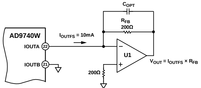
Figure 33. Unipolar Buffered Voltage Output
