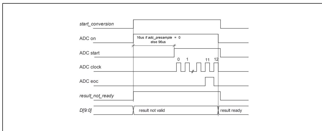
Figure 75: ADC Timing Diagram
