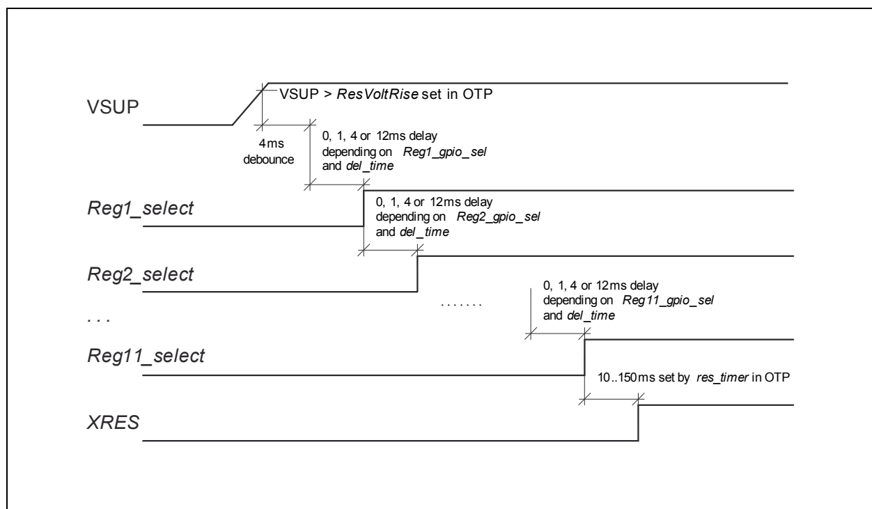
Figure 57: Regulator Power-Up Sequence
