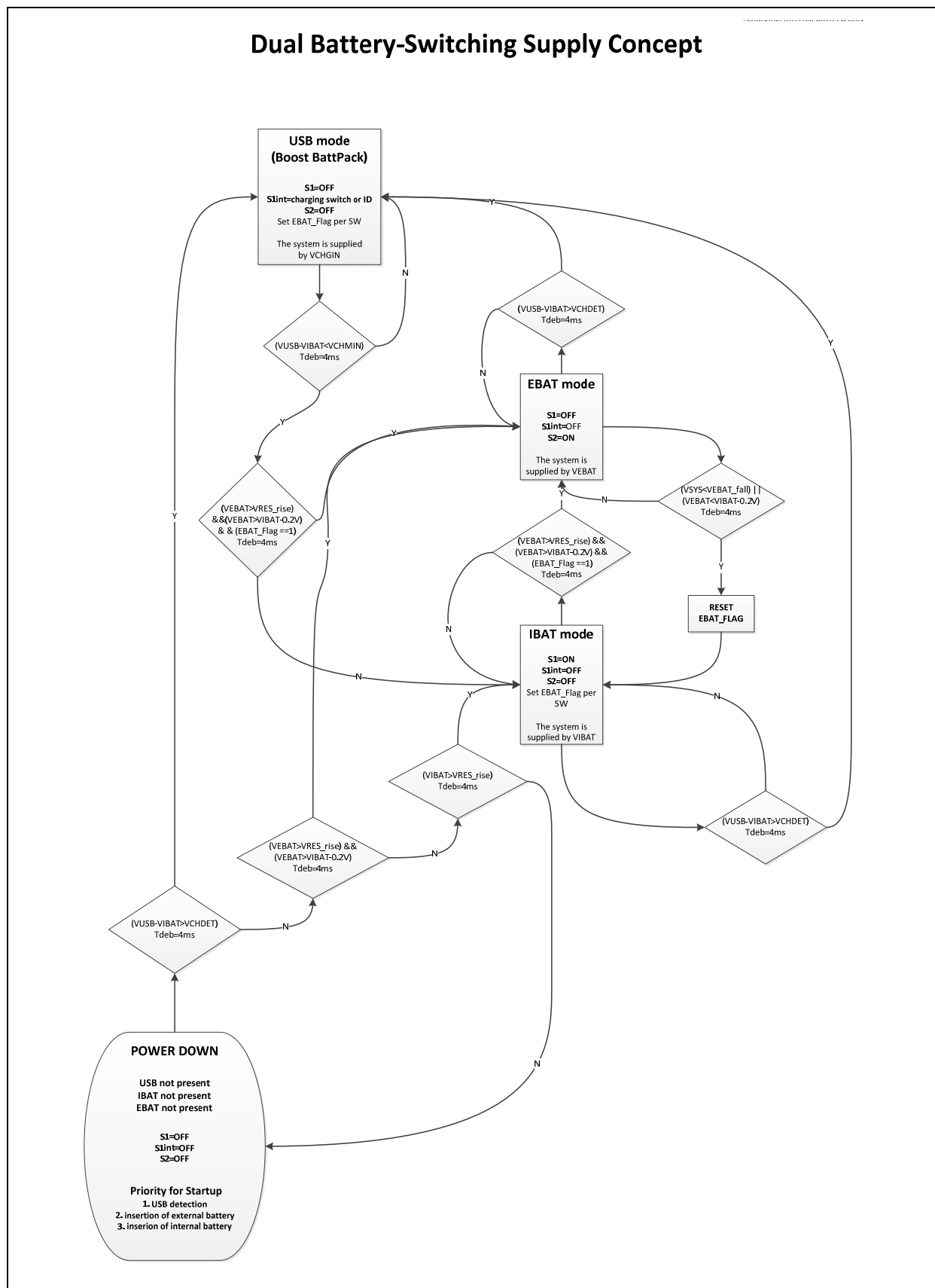
Figure 50: Dual Battery Switching (Flowchart)
