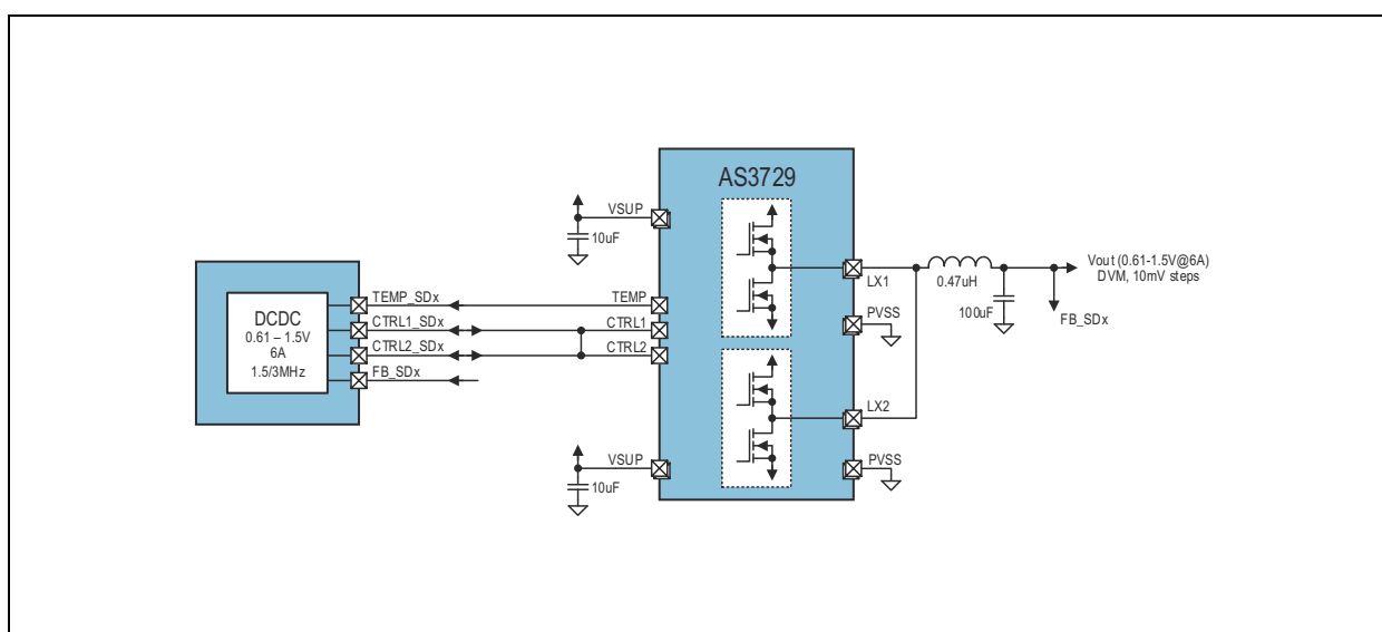
Figure 18: SD4 DC/DC Buck Controller 6A Combined Mode
