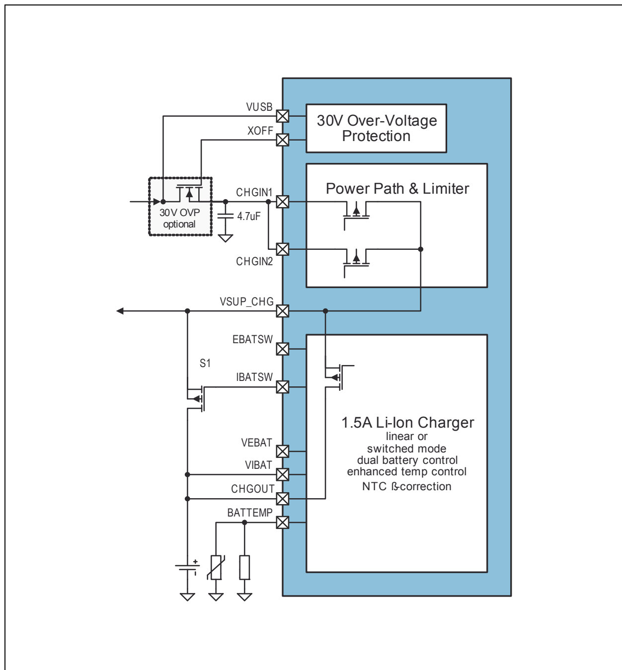
Figure 44: Charger Application Block Diagram, Linear Mode Single Power-Path and Battery
