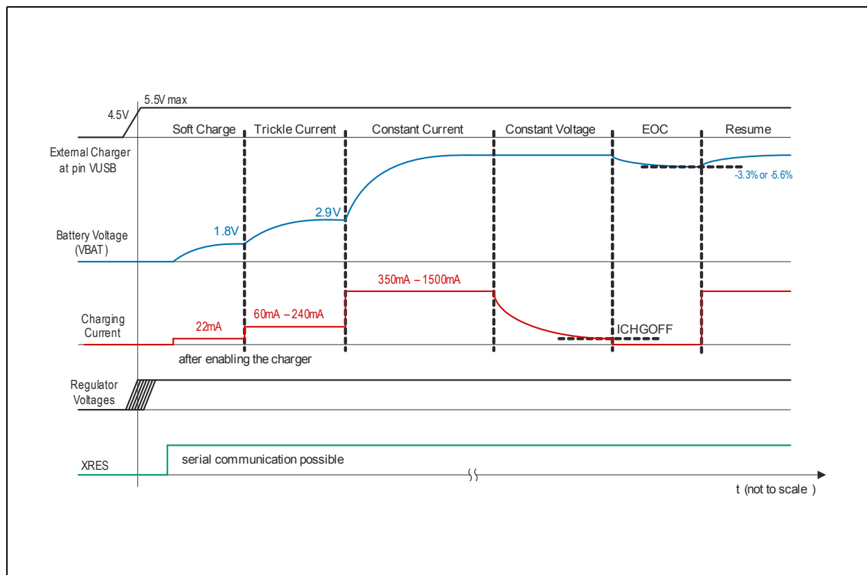
Figure 45: Charger States
