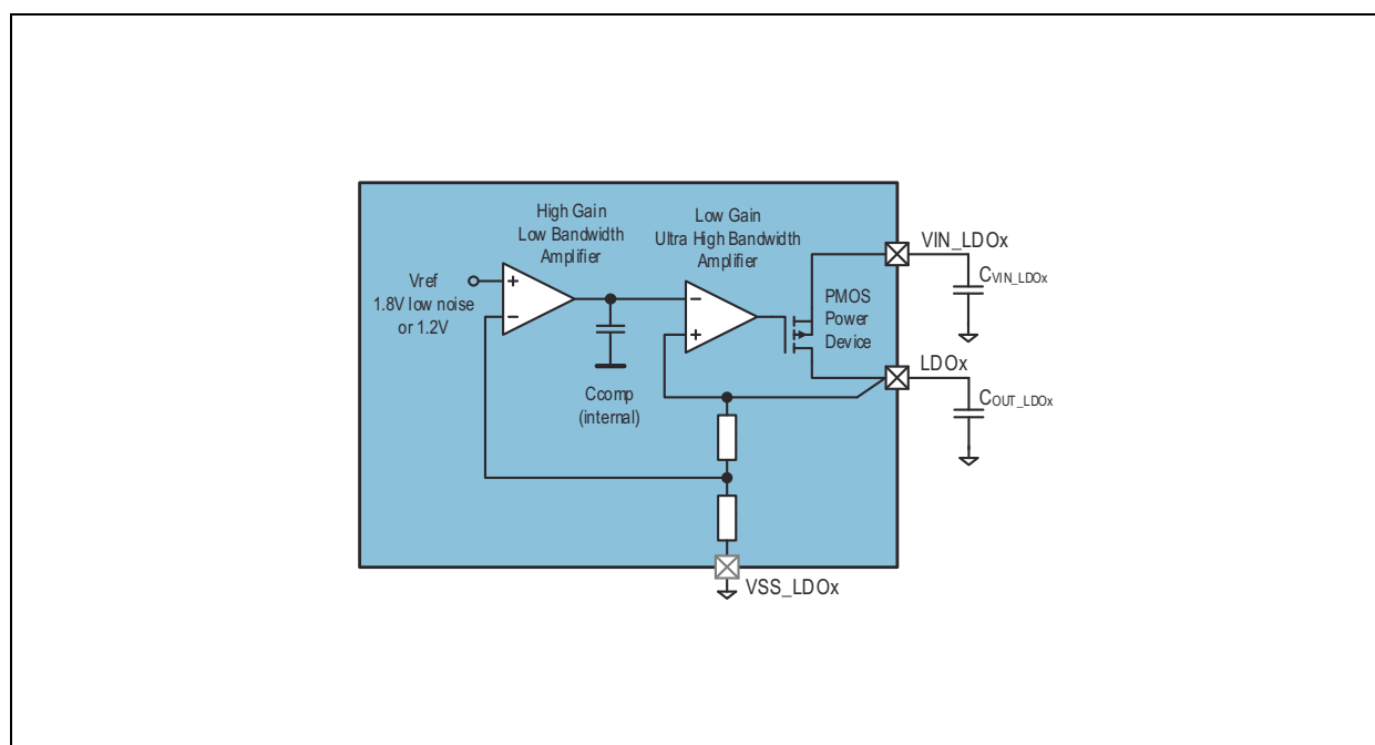
Figure 27: Analog IO LDO Block Diagram
