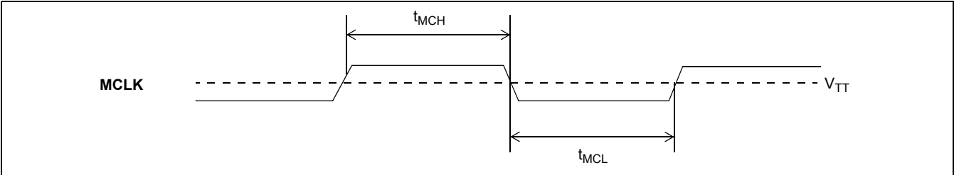
Figure 14 - Master Clock
