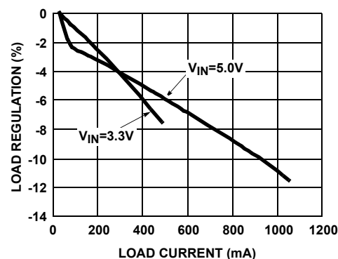
FIGURE 4. BOOST LOAD REGULATION vs LOAD CURRENT (P MODE)
