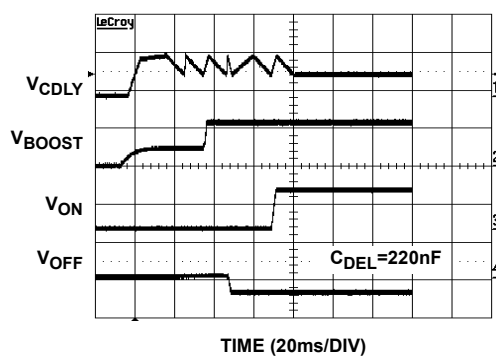
FIGURE 12. START-UP SEQUENCE
