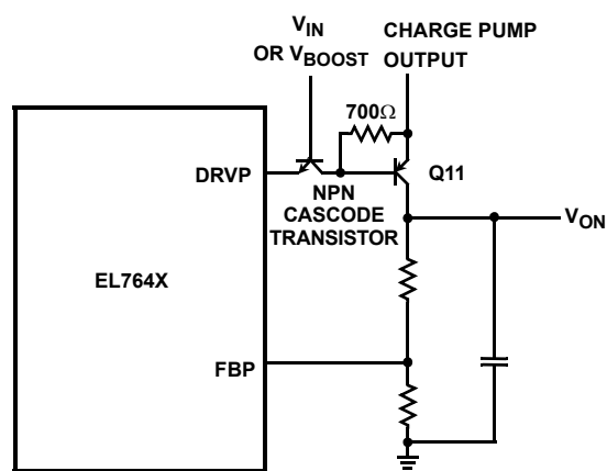
FIGURE 21. CASCODE NPN TRANSISTOR CONFIGURATION FOR HIGH CHARGE PUMP OUTPUT VOLTAGE (&gt;36V)
