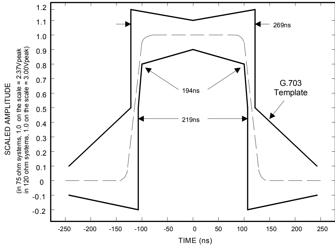
Figure 7-4. E1 Transmit Pulse Template
