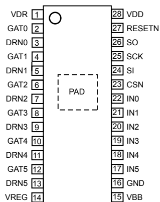
Pinout Diagram
