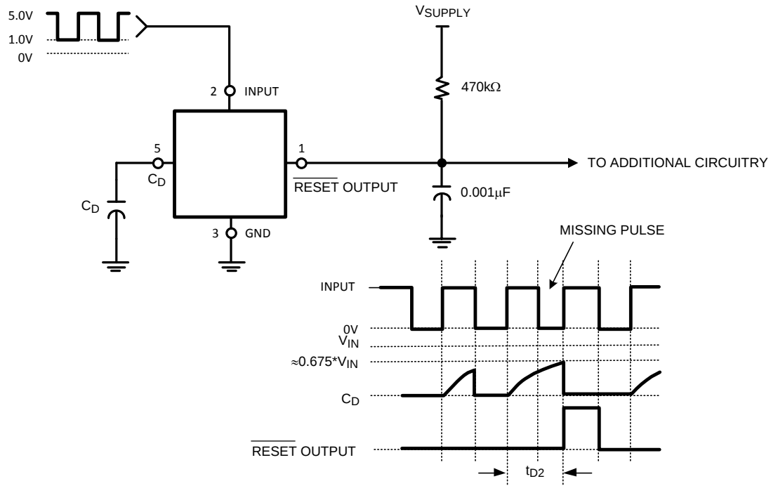
Figure 17. Missing Pulse Detector Using LM8365BALMF45
