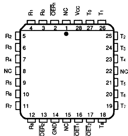
PLCC
