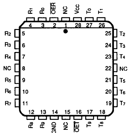
PLCC
