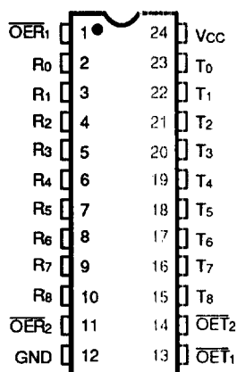
DIP*
