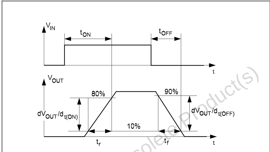
Figure 5. Turn-ON and turn-OFF
