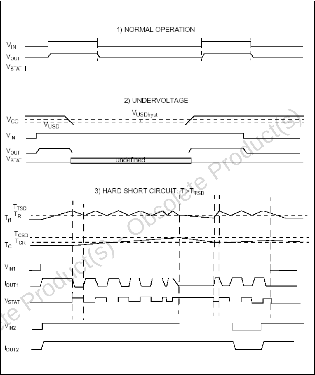
Figure 7. Waveforms
