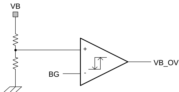
Figure 26. VB Monitor Block Diagram
