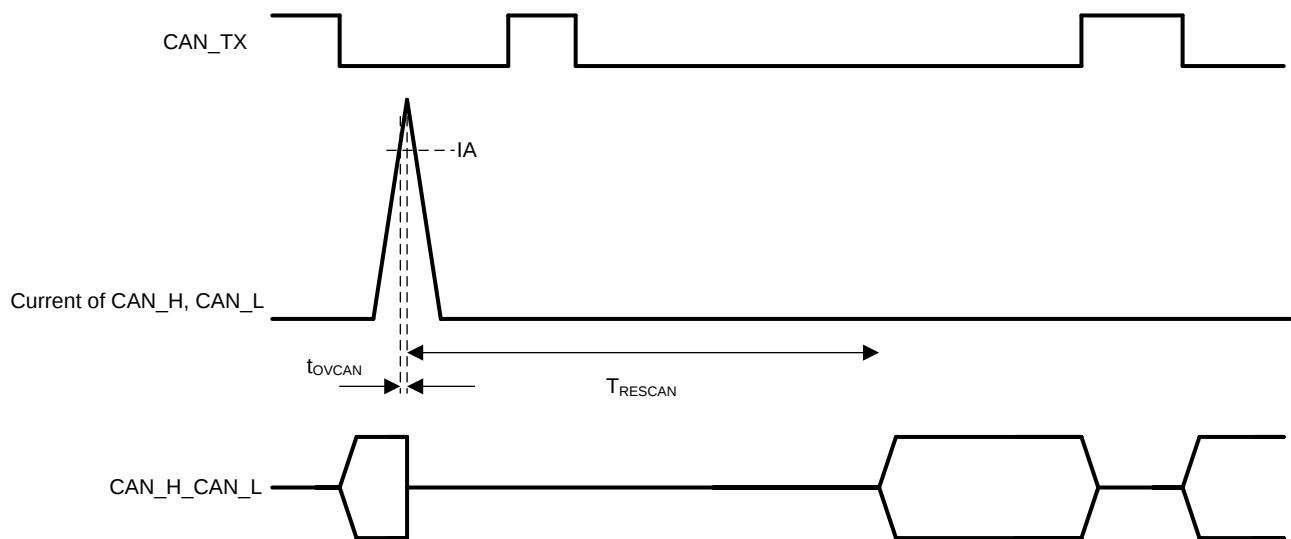
Figure 6. Overcurrent Event
