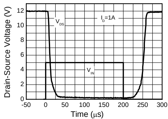
Switching Speed
