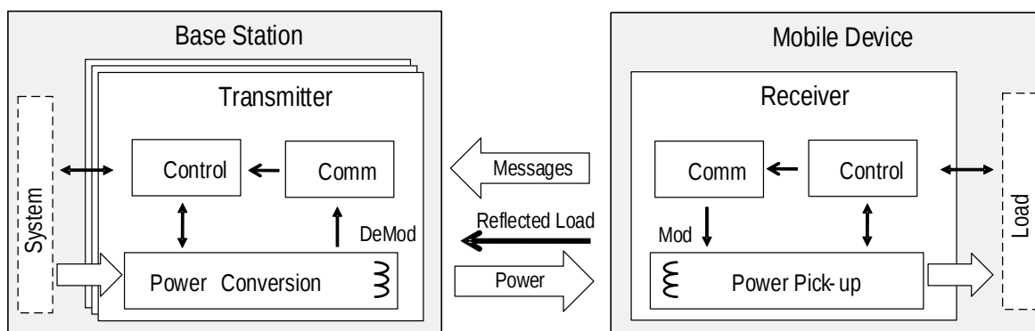
Figure 2. Block Diagram of WPC System
