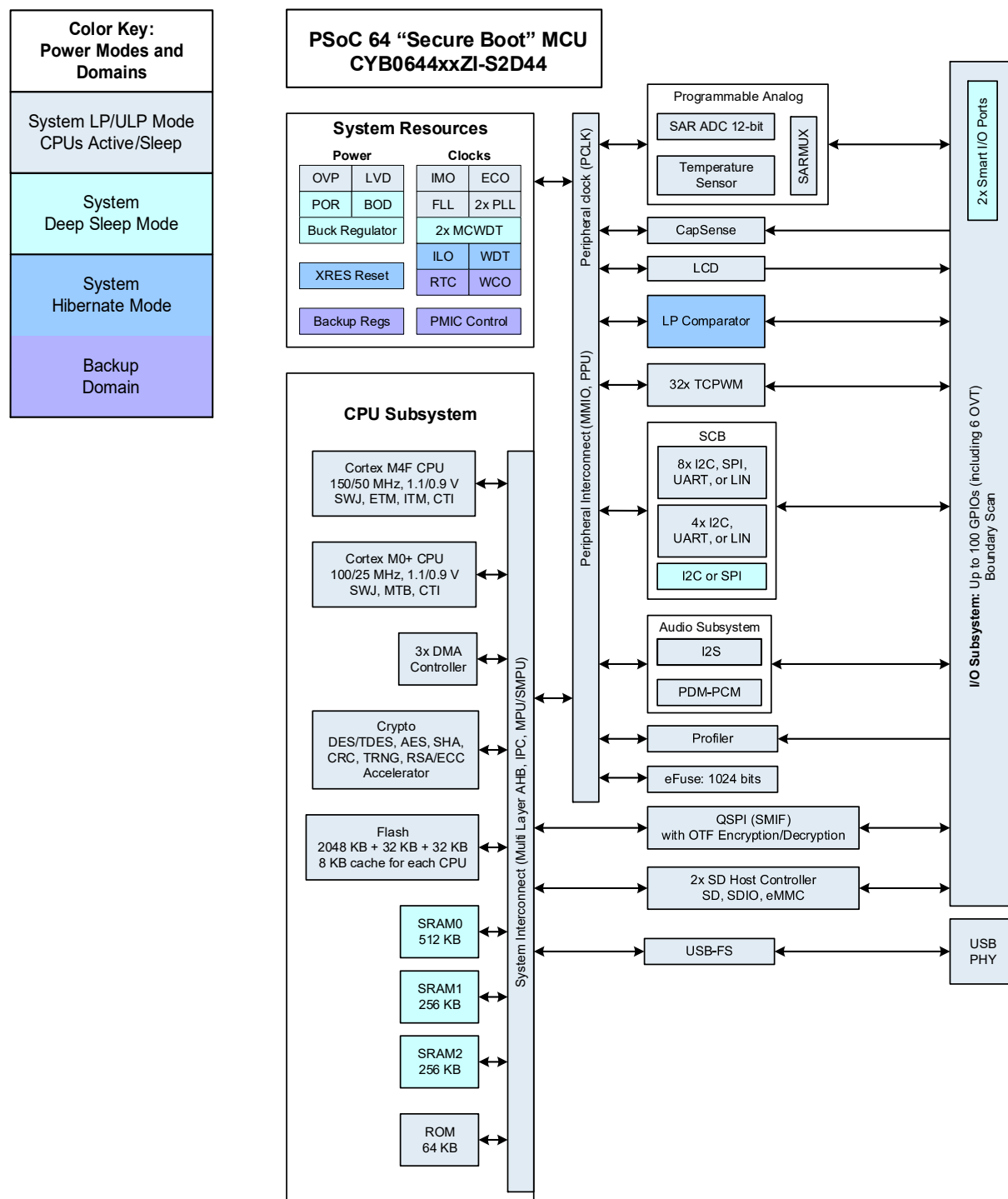
Figure 2. Block Diagram
