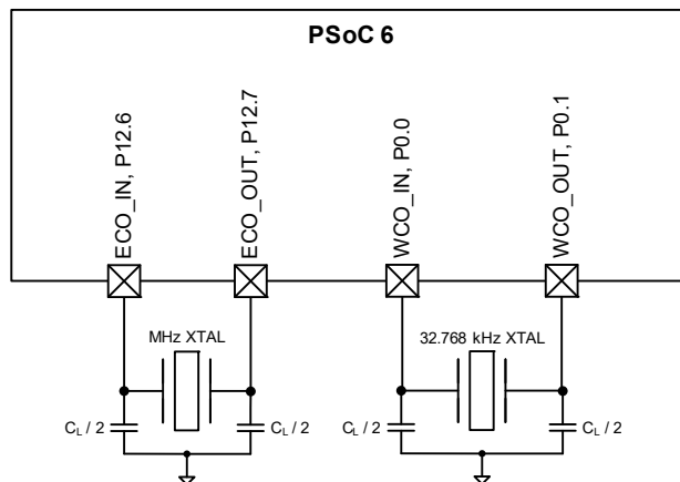
Figure 4. Oscillator Circuits
