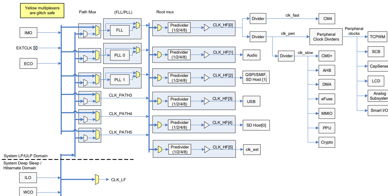
Figure 3. Clocking Diagram
