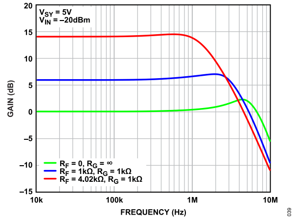
Figure 40. Noninverting Small Signal Frequency Response
