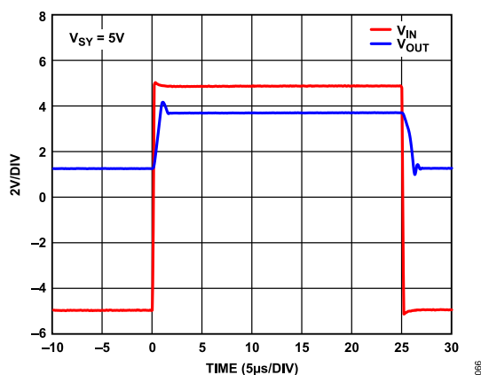
Figure 71. \pm 10 V to 0 V to +5 V Funnel Amplifier, Large Signal Pulse Response
