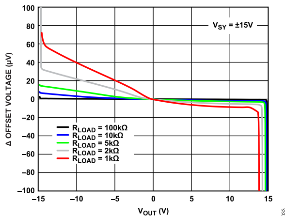
Figure 34. \Delta Offset Voltage vs. Output Voltage ( V_{OUT} )
