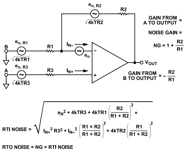
Figure 62. Op Amp Noise Analysis Model
