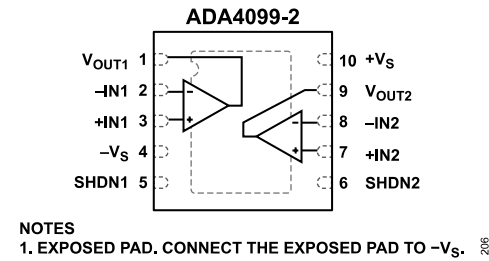
Figure 6. Pin Configuration for ADA4099-2 10-Lead LFCSP
