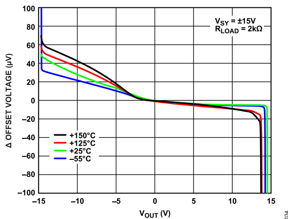
Figure 35. \Delta Offset Voltage vs. V_{OUT} (2 k \Omega Load)
