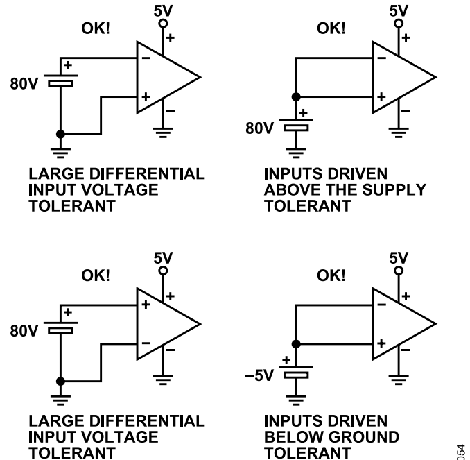
Figure 57. ADA4099-1 and ADA4099-2 Fault Tolerant Conditions
