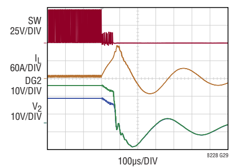
BG MOSFET Short in Regulation (Boost)
