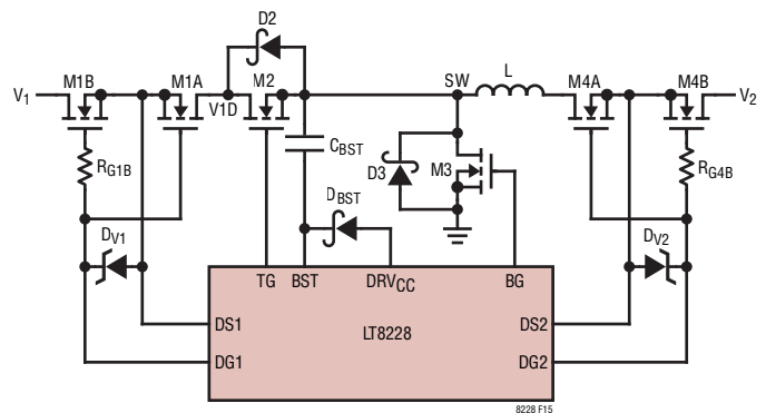
Figure 15. Power MOSFETs and Components Selection
