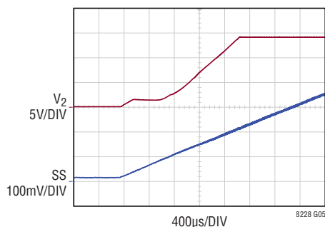
Soft Start-Up (Buck)
