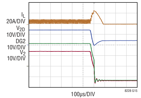
Reverse Battery Insertion at V_2 in Regulation
