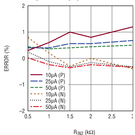
IMON2 Gain Error vs R_{IN2} ( V_{CM2} > 2.5\text{V} , Output: 10\mu\text{A} , 25\mu\text{A} and 50\mu\text{A} )
