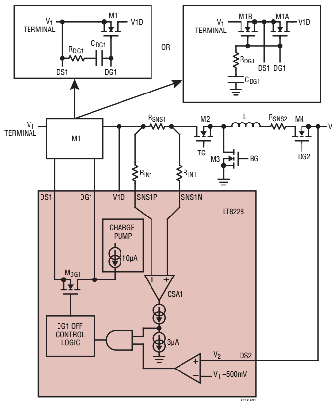
Figure 1. M1 Control in Buck Mode
