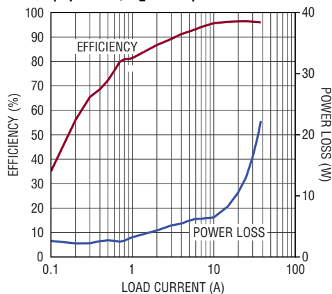
Efficiency vs V_2 Current (Buck) ( V_1 = 48\text{V} , V_2 = 14\text{V} )
