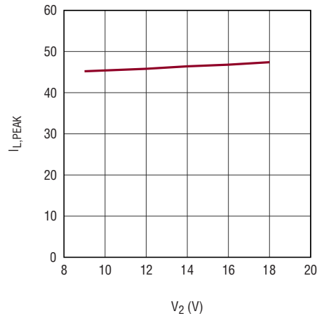
Maximum Inductor Current vs V_2 (Boost)
