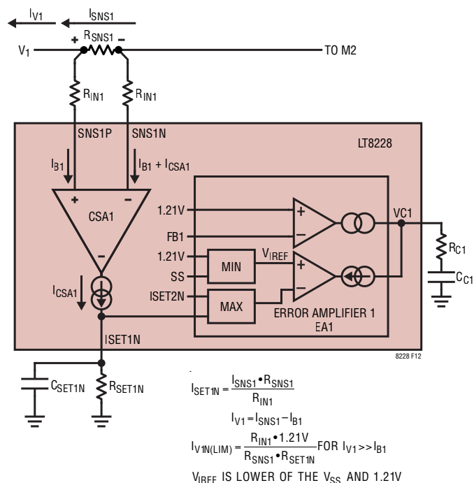
Figure 12. V_1 Output Current Limit Programming at ISET1N
