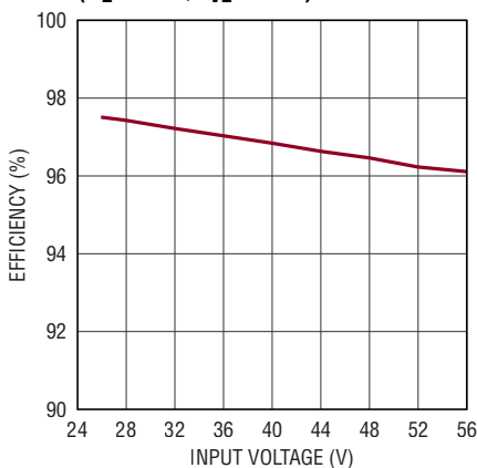
Efficiency vs V_1 (Buck) ( V_2 = 14\text{V} , I_{V2} = 20\text{A} )
