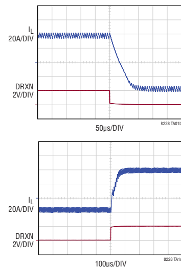
Buck and Boost Mode Transitions
