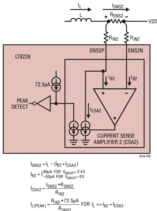
Figure 6. V_2 Current Sense Amplifier Operation for Positive Inductor Current
