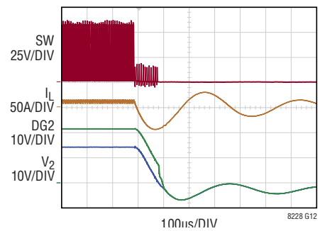
BG MOSFET Short in Regulation (Buck)
