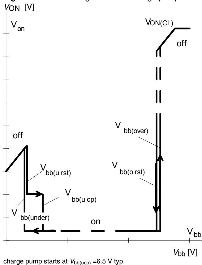
Figure 7a: Overvoltage:
