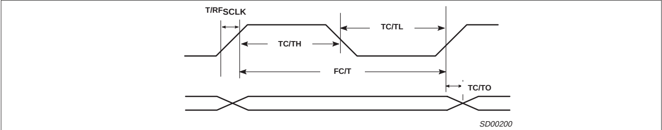
Figure 9. Counter/Timer Baud Rate Clock, External
