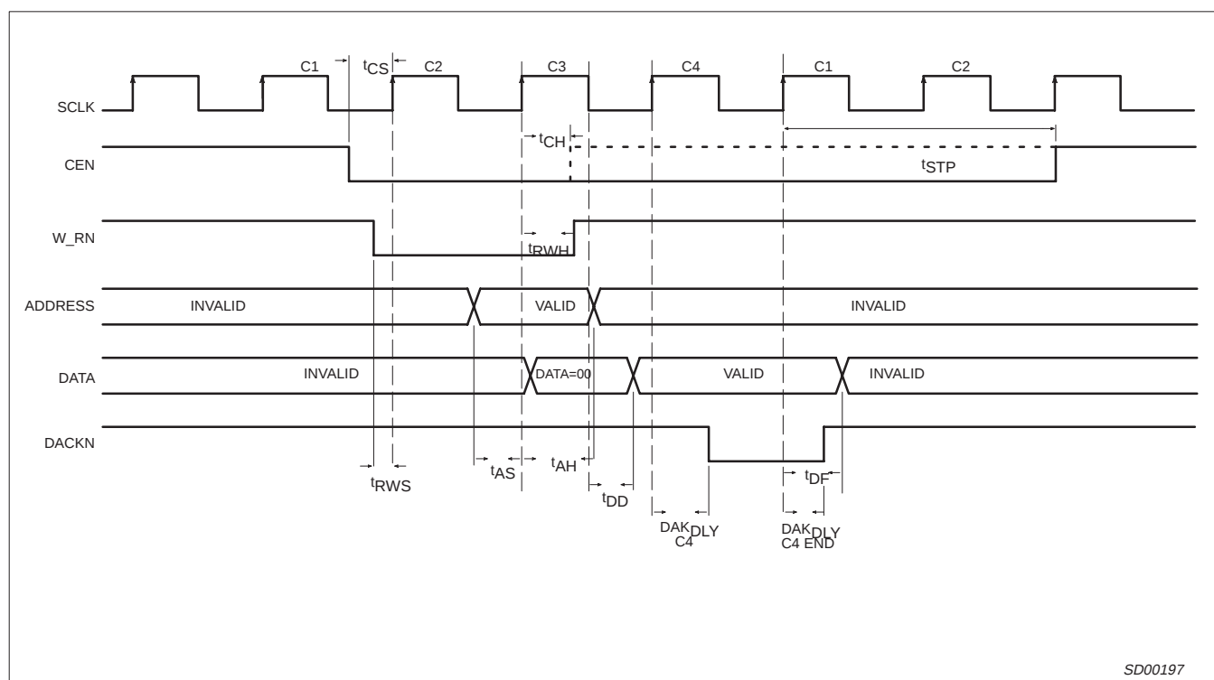
Figure 5. Basic Read Cycle, SYNC
