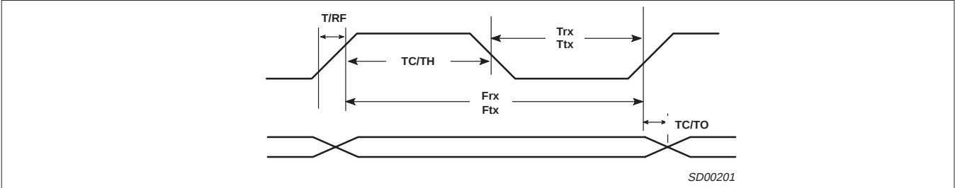
Figure 10. Tx/Rx Clock Timing, External
