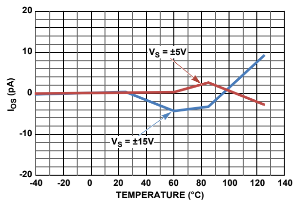
FIGURE 8. ISL28110 INPUT OFFSET CURRENT ( I_{OS} ) vs TEMPERATURE
