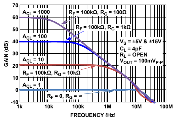
FIGURE 50. CHARACTERIZED CLOSED LOOP GAIN vs FREQUENCY
