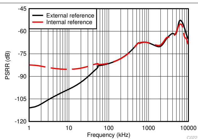
Figure 6-22. PSRR vs Frequency
