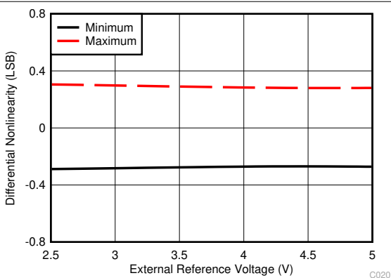
Figure 6-7. DNL vs External Reference Voltage
