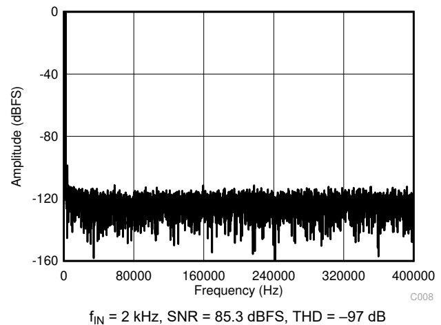
Figure 6-14. Typical FFT
