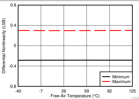
Figure 6-3. Typical DNL
