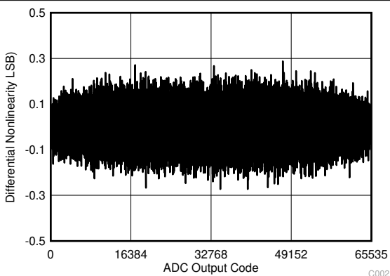
Figure 6-3. Typical DNL
