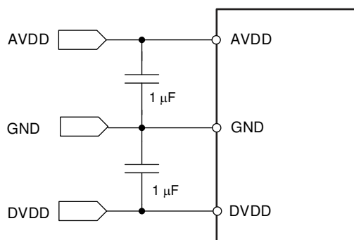
Figure 9-1. Power-Supply Decoupling
