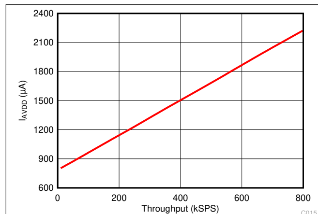
Figure 6-21. Analog Supply Current vs Throughput
