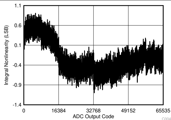
Figure 6-4. Typical INL
