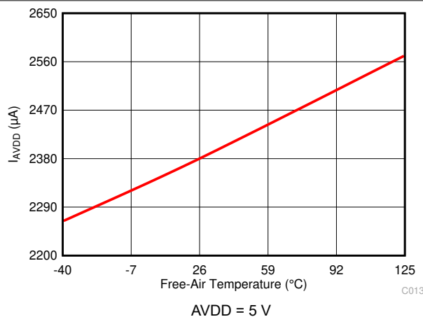
Figure 6-19. Analog Supply Current vs Temperature
