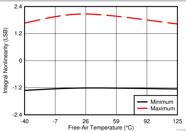
Figure 6-4. Typical INL
