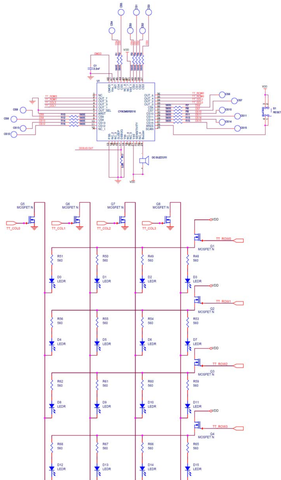
Figure 3. Schematic 2: 16 Buttons with Truth Table Output Mode
