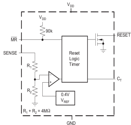
Fixed Voltage Diagram
