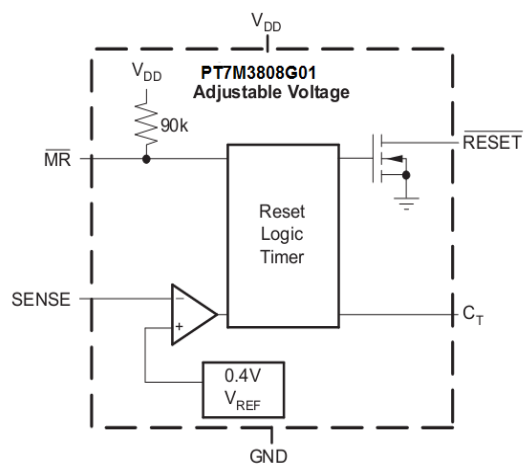
Adjustable Voltage Diagram (PT7M3808G01)
