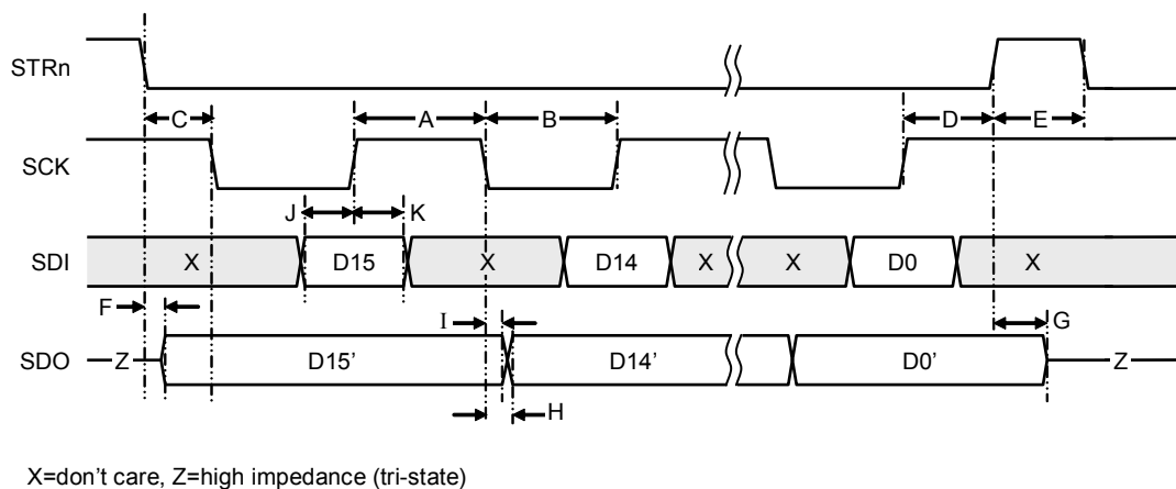
Figure 4: Serial Interface Timing
