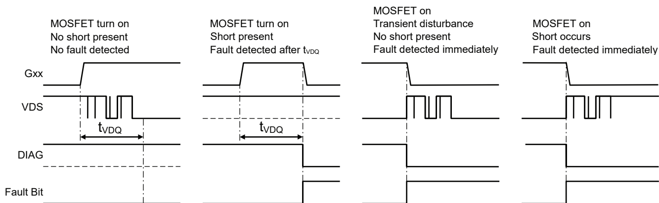
Figure 7: VDS Fault Monitor – Blank Mode Timing (VDQ = 1)
