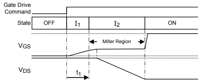
Figure 13a: Off-to-On Transition (Gate Drive Control)
