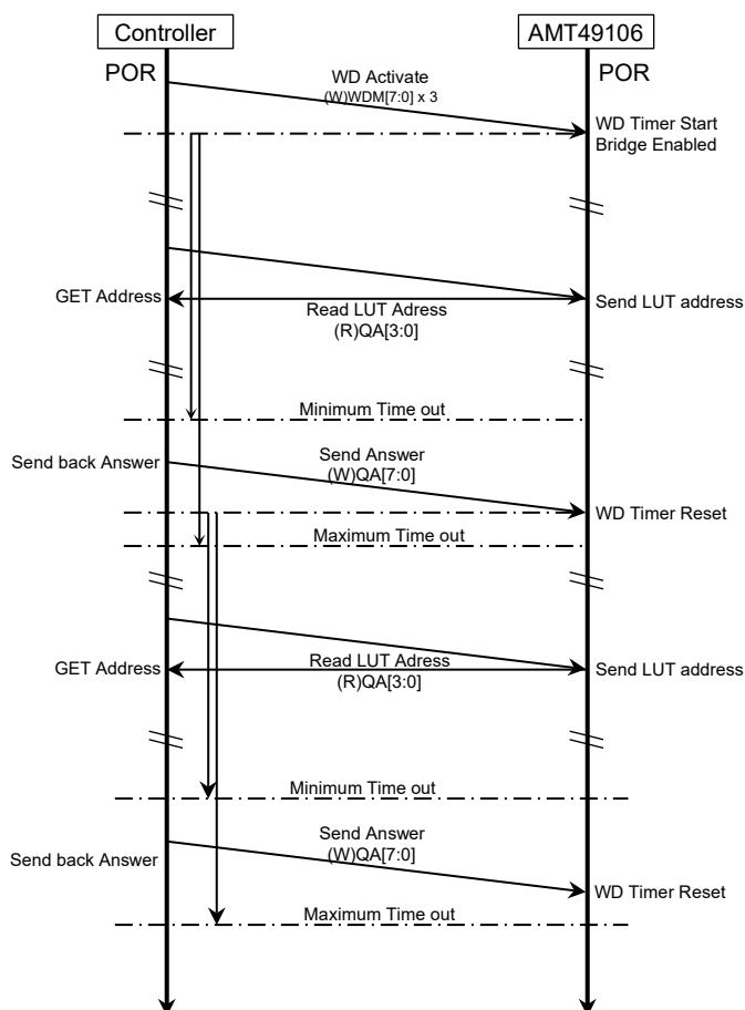
Figure 15: Q&A Communication Sequence
