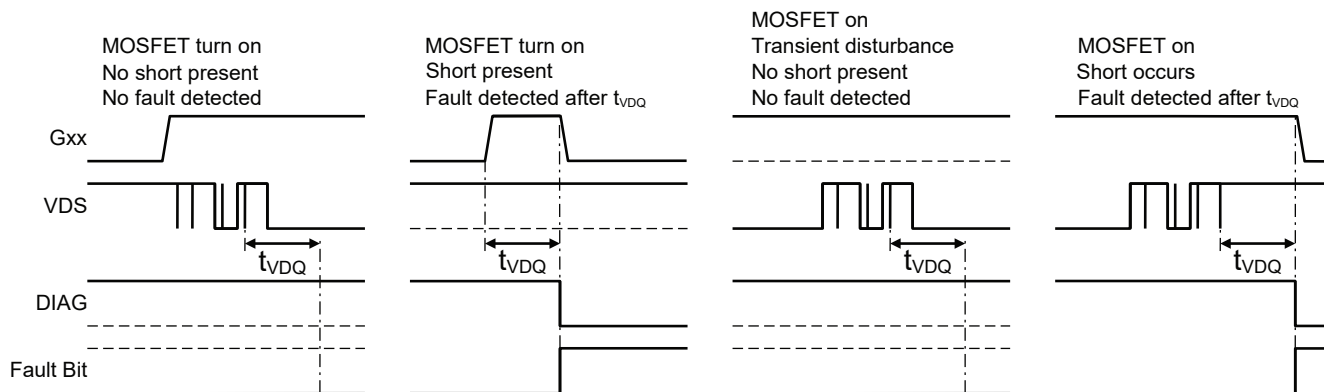
Figure 8: VDS Fault Monitor – Debounce Mode Timing (VDQ = 0)
