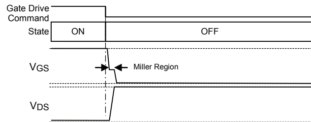
Figure 13d: On-to-Off Transition (Switched)
