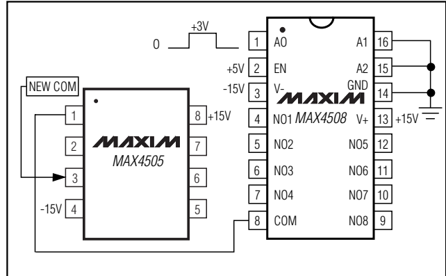
Figure 4. Demultiplexer Application Using MAX4505 with MAX4508
