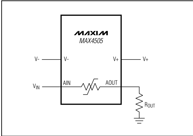
Figure 2. Application Circuit
