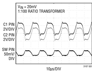
Resonant Switching Waveforms
