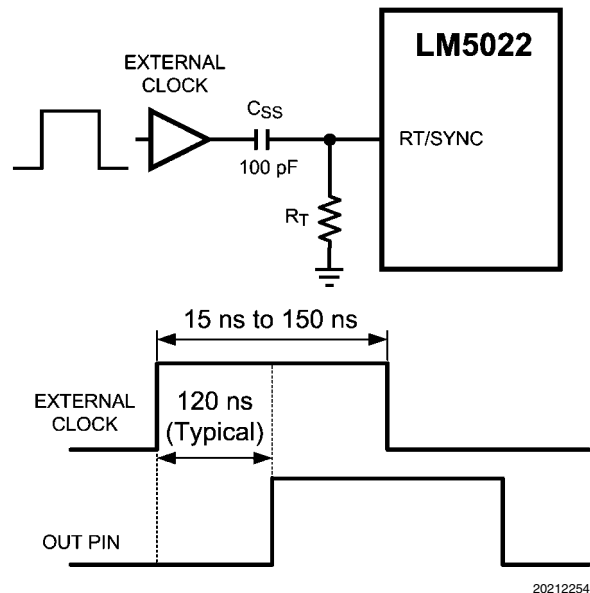
FIGURE 3. Sync Operation
