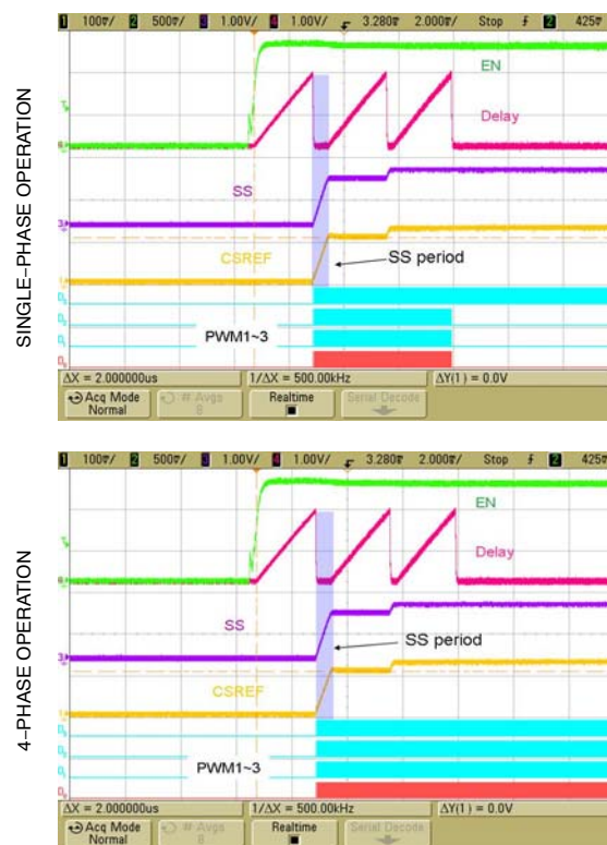
Figure 6. Typical Startup Waveform 1-Vo, 2-EN, 3-SS, 4-DELAY, D0-D3-PWM1~4
