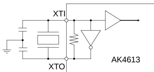
Figure 18. X'tal mode
