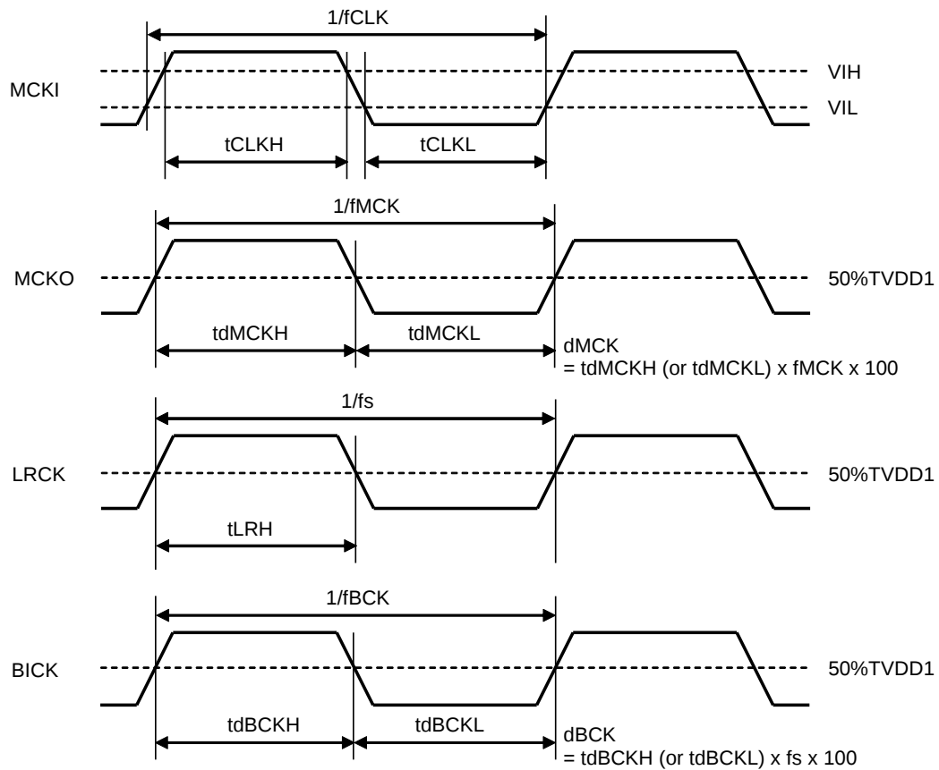
Figure 6. Clock Timing (Except TDM1/0 bit = "00" &amp; Master mode)
