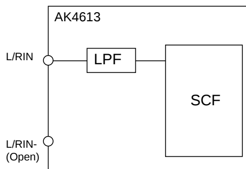
Figure 20. Single-end Input (DIE1-2 bit = “0”)
