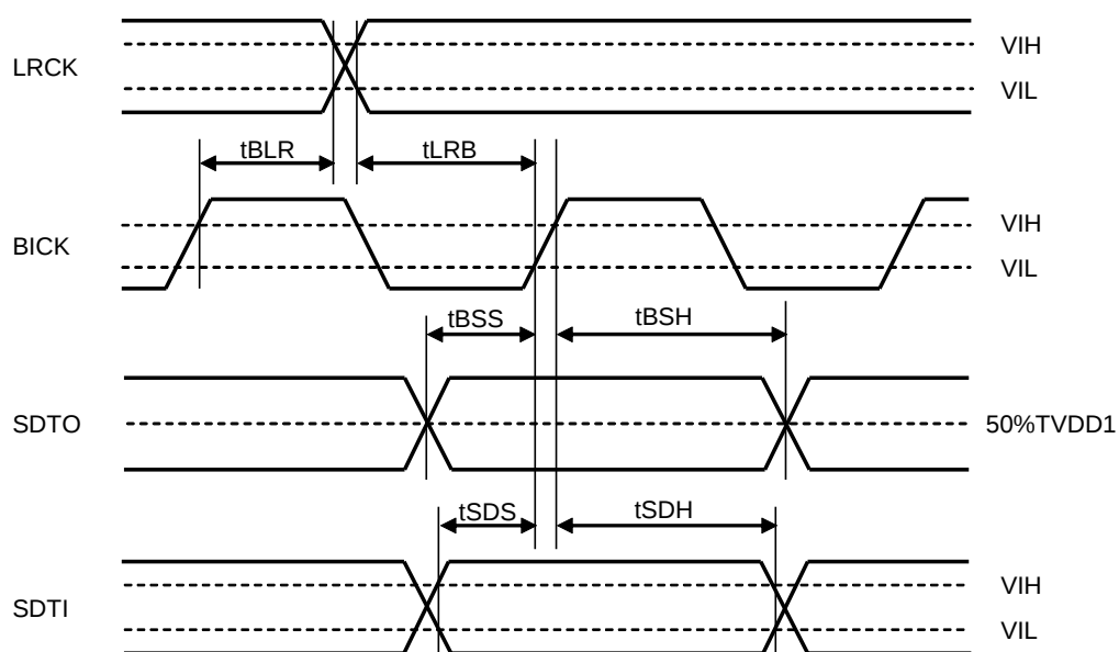
Figure 8. Audio Interface Timing (Except TDM1/0 bit = "00" &amp; Slave mode)
