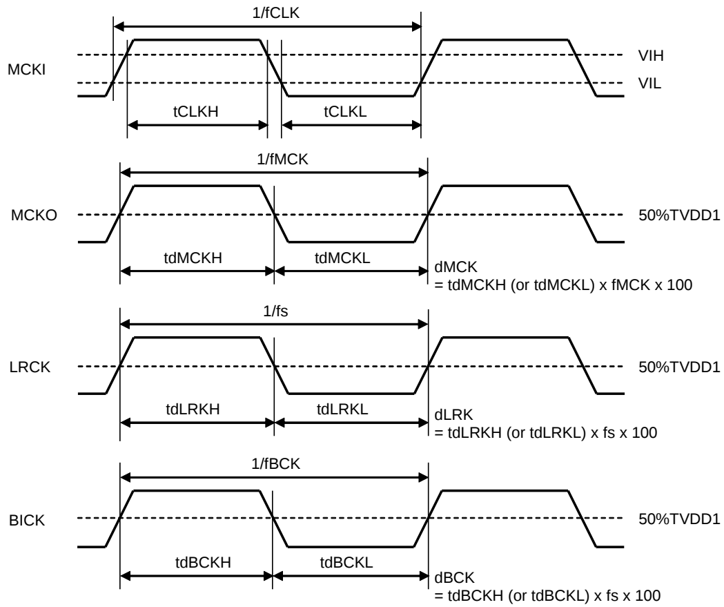
Figure 5. Clock Timing (TDM1/0 bit = "00" &amp; Master mode)
