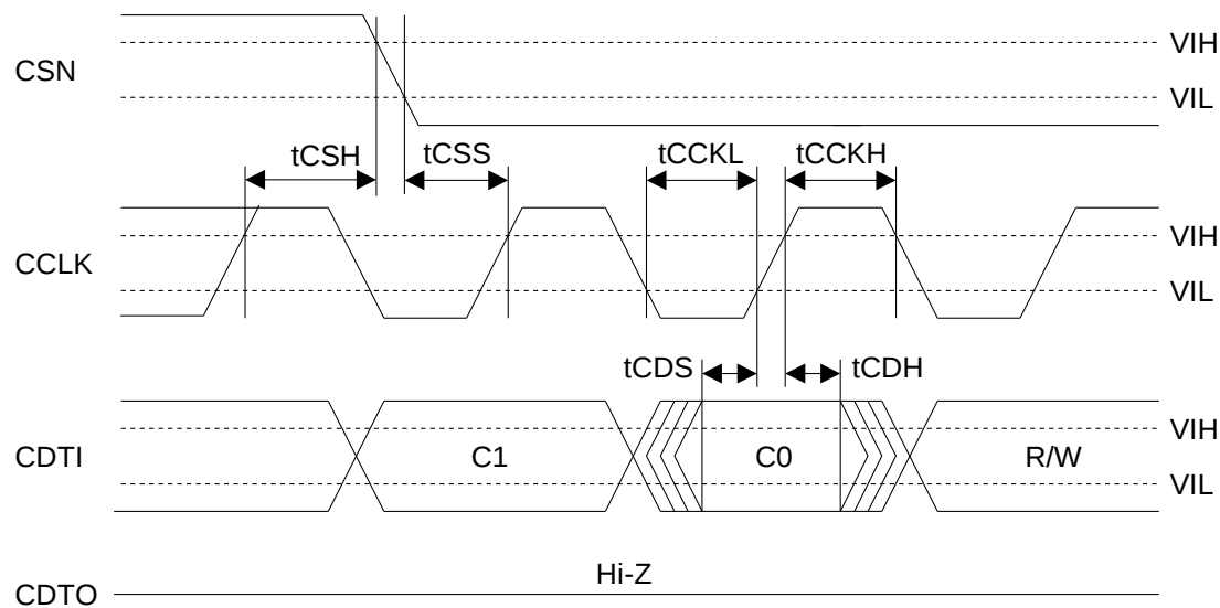
Figure 11. WRITE Command Input Timing (4-wire Serial mode)
