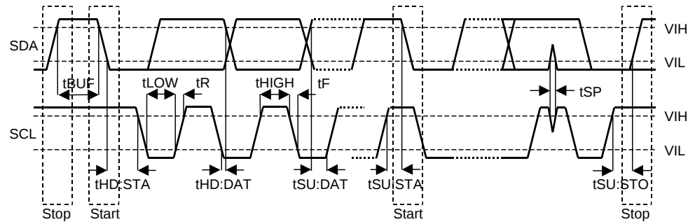
Figure 15. I²C Bus mode Timing
