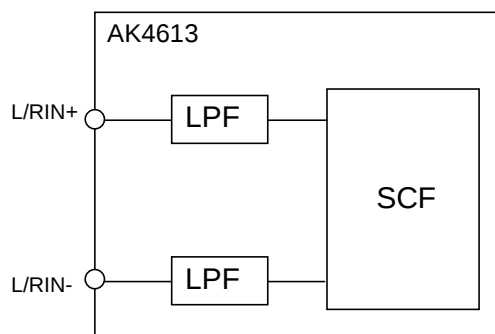
Figure 19. Differential Input (DIE1-2 bit = “1”)
