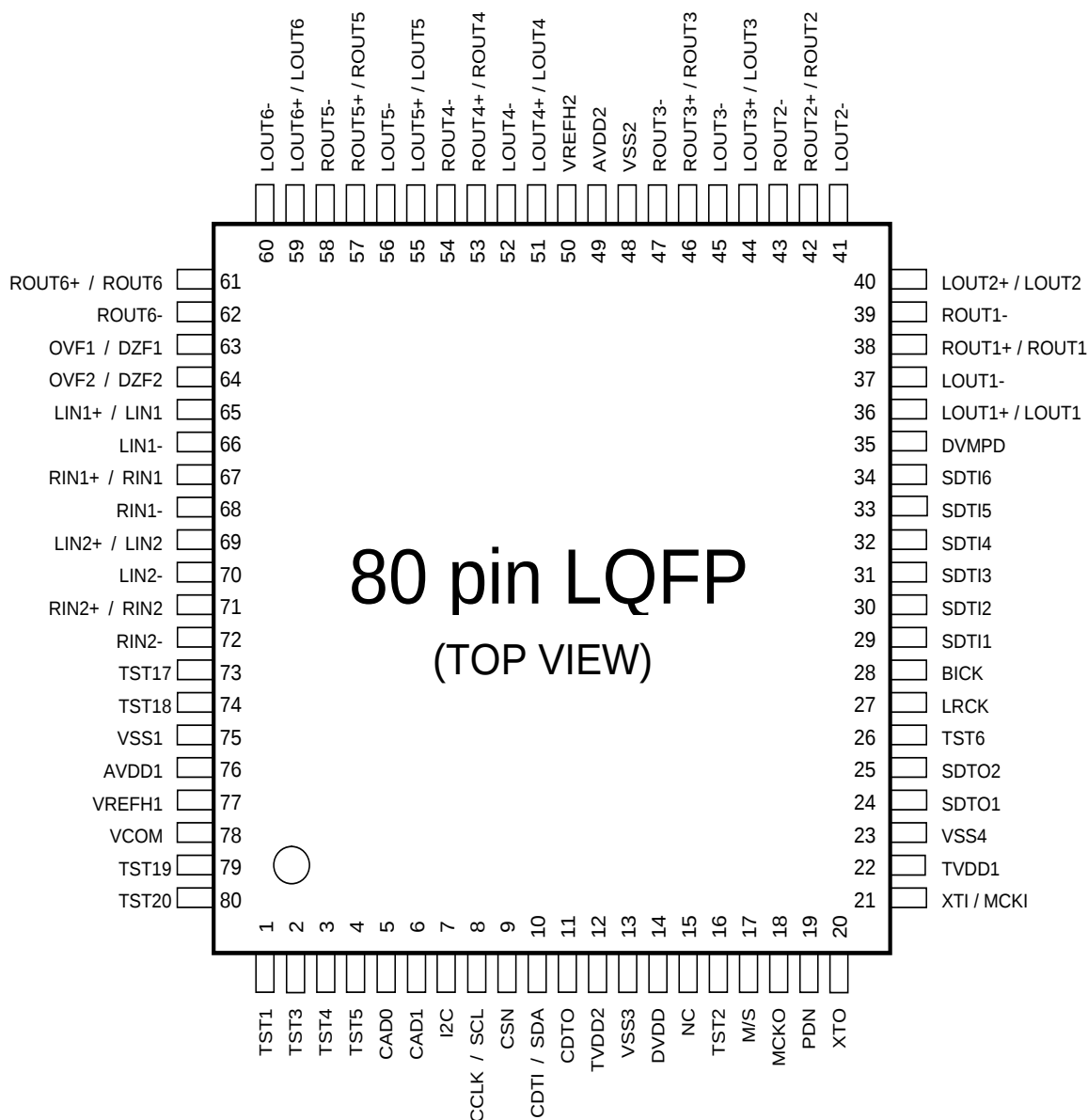
Figure 2. Pin Layout
