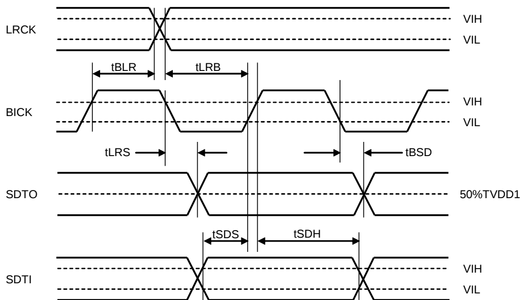
Figure 7. Audio Interface Timing (TDM1/0 bit = "00" &amp; Slave mode)
