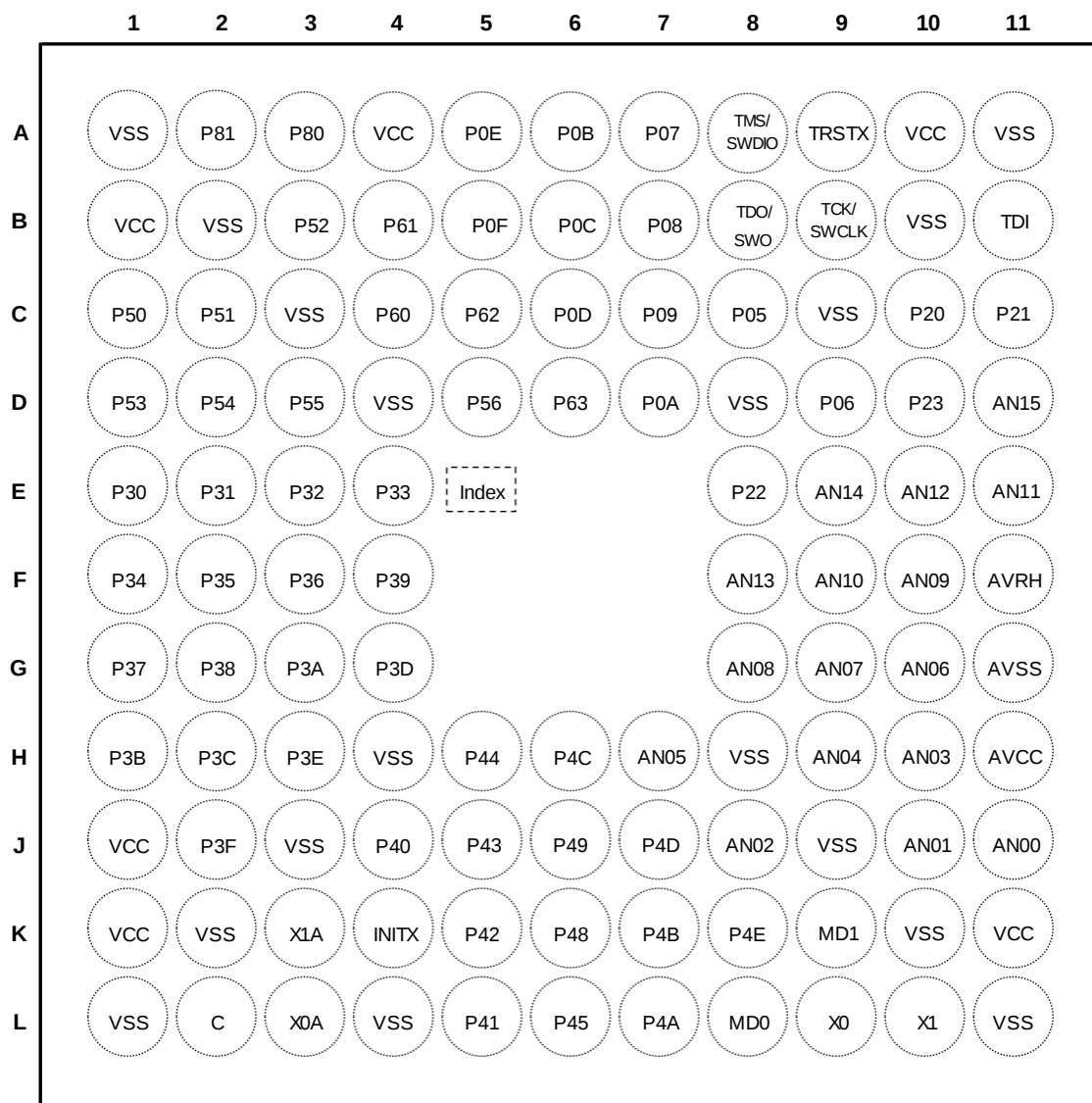
(TOP VIEW)
