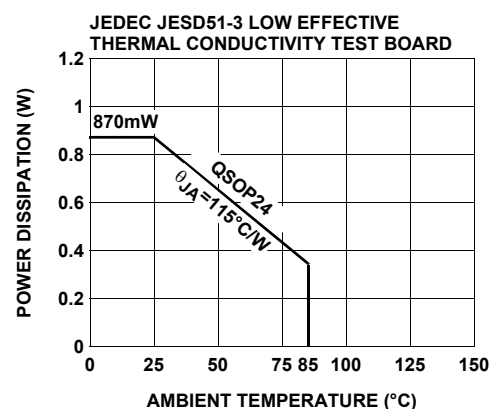
FIGURE 2. PACKAGE POWER DISSIPATION vs AMBIENT TEMPERATURE
