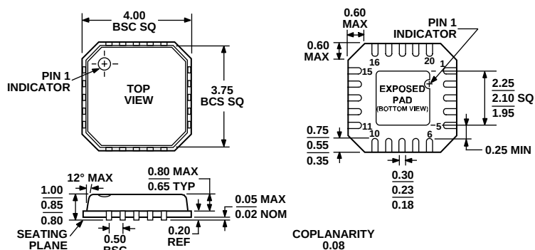
Figure 32. 20-Lead Lead Frame Chip Scale Package [LFCSP_VQ] 4 mm x 4 mm Body, Very Thin Quad (CP-20-1)
