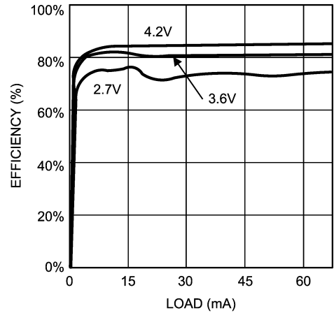
Vsub Efficiency vs. Load ( V_{sub} = 15V )
