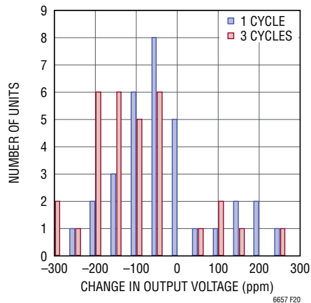
Figure 20. \Delta V_{OUT} Due to IR Reflow, Peak Temperature = 260°C
