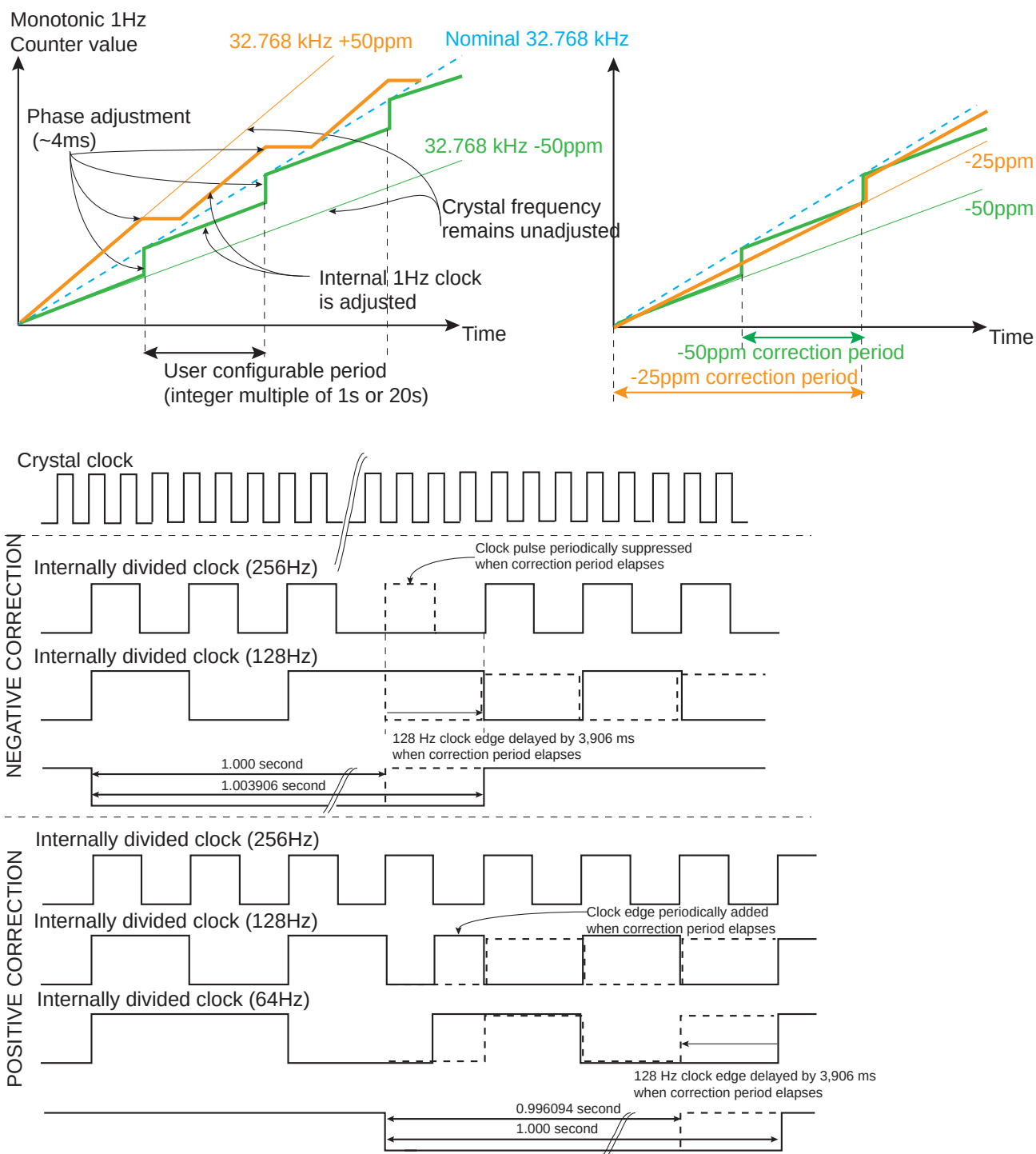
Figure 17-4. Calibration Circuitry Waveforms
