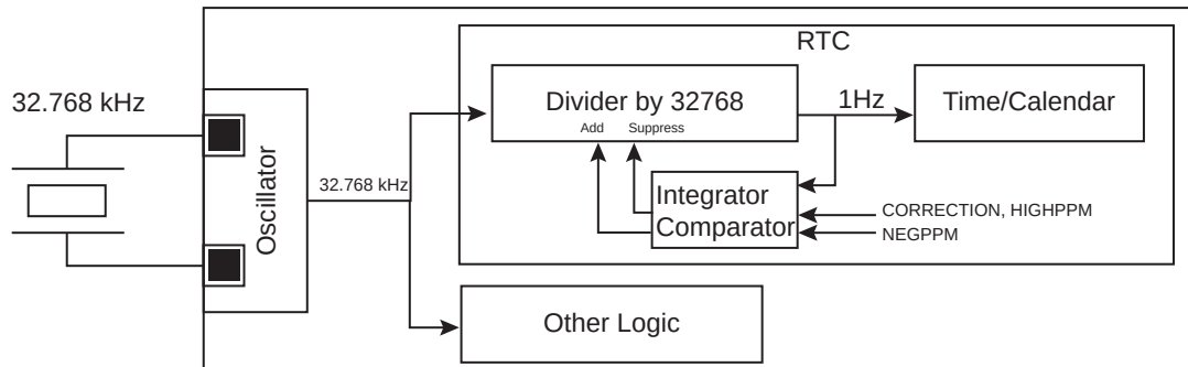
Figure 17-3. Calibration Circuitry
