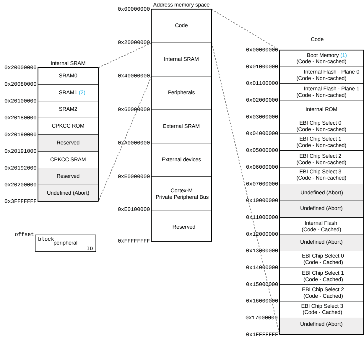
Figure 7-3. SAM4CM32 Memory Mapping of CODE and SRAM Area
