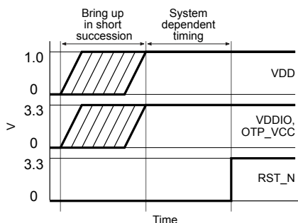
Figure 17: Sequencing of power supplies and RST_N
